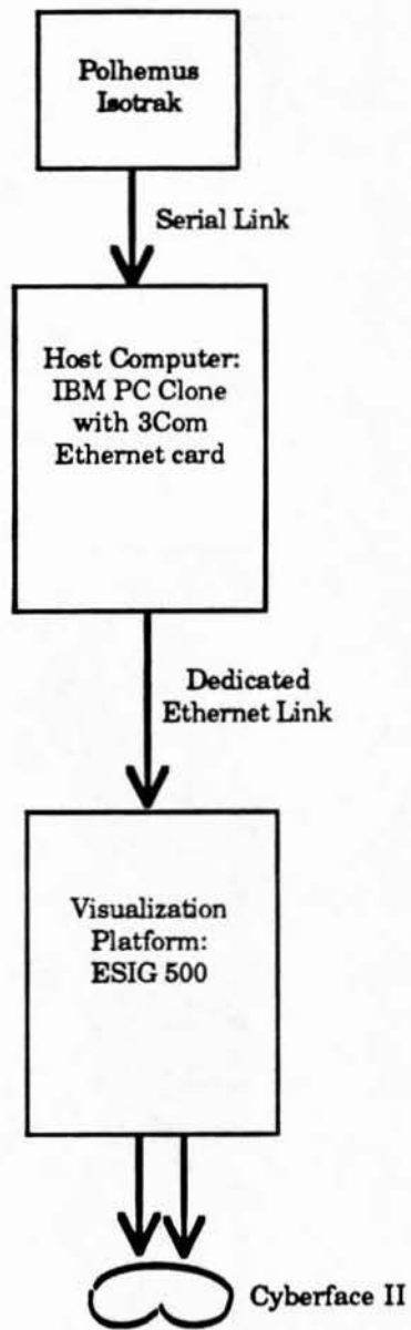
Figure 8: ESIG/CyberFace Configuration
