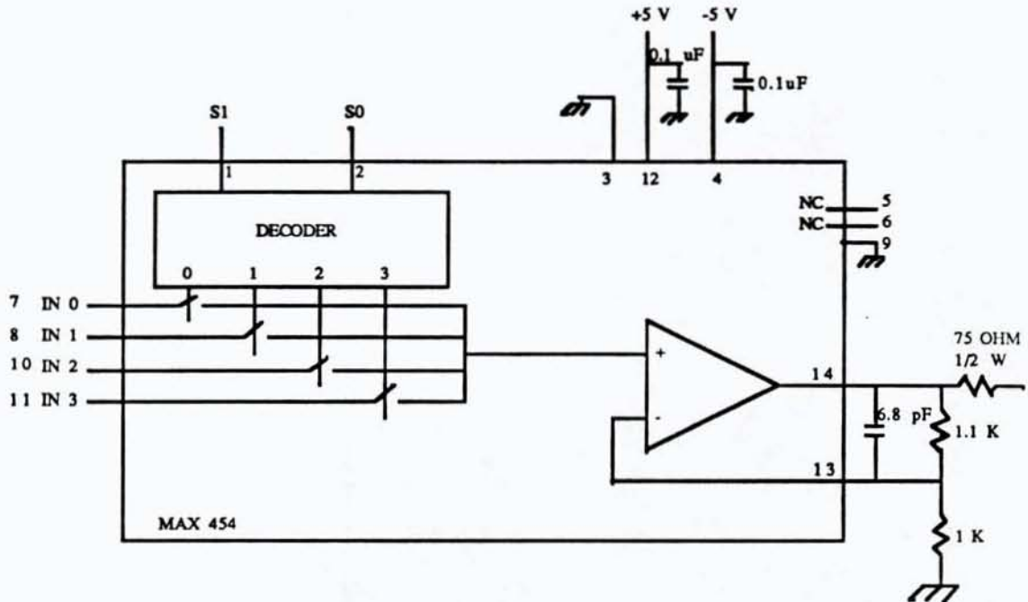
Figure 5: Video Switcher (One module of Six). Functional Diagram
