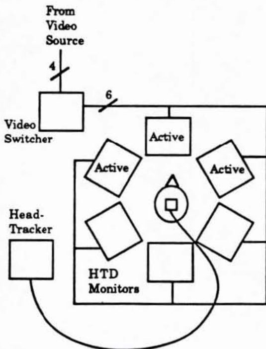
Figure 1. The Head-Tracking Display (HTD)
