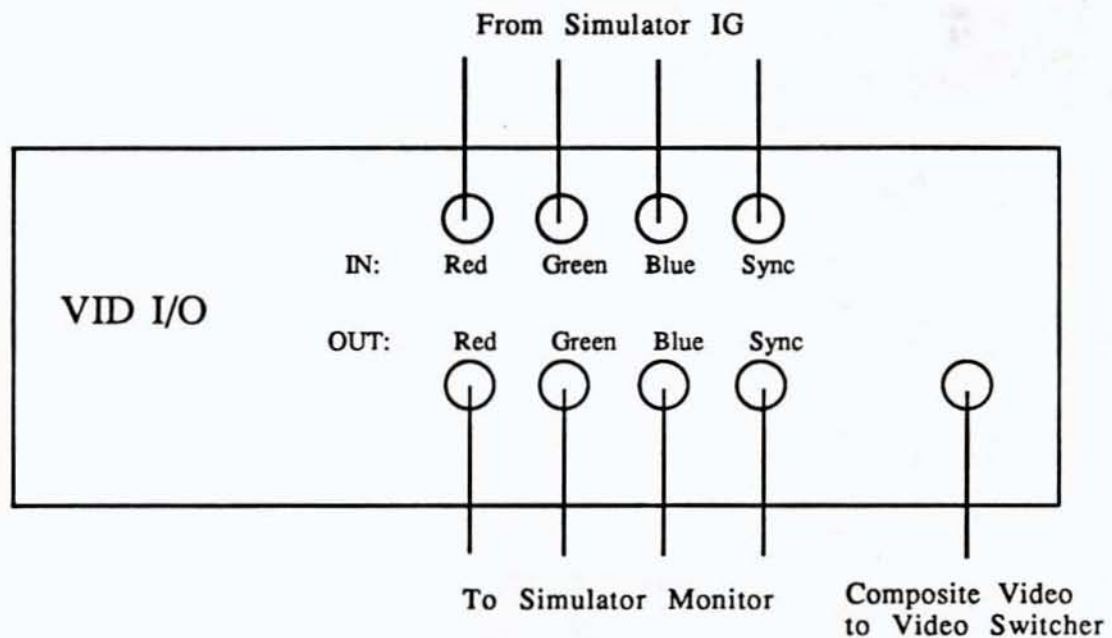
Figure 3. VID I/O Video Encode (x three)
