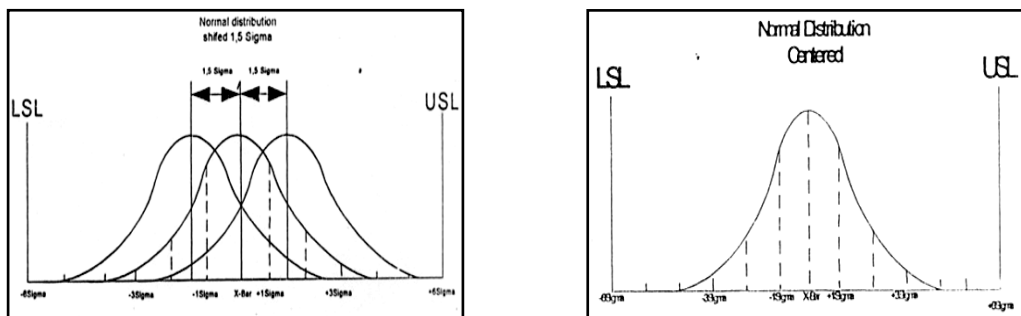
Sumber : William J. Kolarik, Creating Quality : Process Design for Results,WCB/McGraw-Hill, Singapore, 1999, hal. 537 Gambar 2.1. Gambar 2.2. True 6-Sigma process, Konsep Six Sigma Motorola dengan pergeseran \pm 1,5 sigma.
