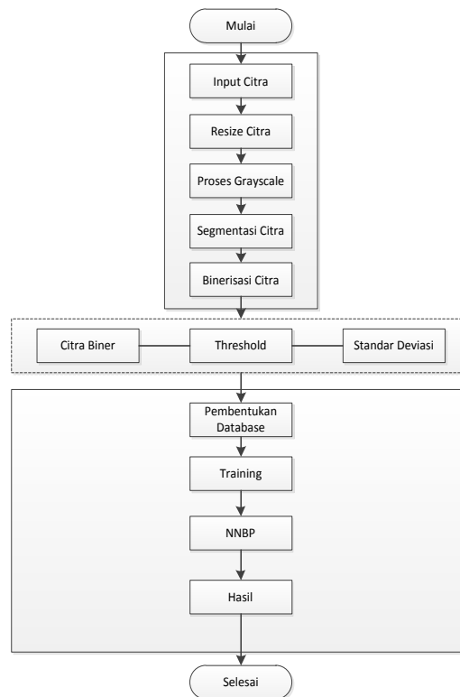
Gambar 2. Flowchart system
