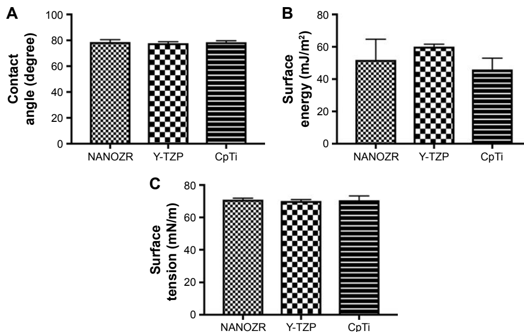
Figure 4 Surface wettability of NANOZR, Y-TZP and CpTi.
