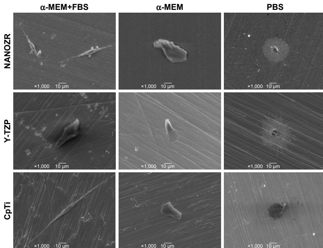
Figure 6 Scanning electron microscopy observation of MC3T3-E1 cells cultured in three different culture media: PBS, \alpha -MEM, and \alpha -MEM supplemented with 10% FBS, on all surfaces after 24 hours of incubation. Magnification: 1,000 \times .
