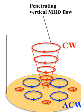
Fig. 3. Schematic of the reversal of the vertical MHD flow near the electrode surface in the tube wall.
