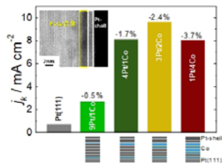
Fig.1 ORR activity for the Pt-Co model catalysts.
