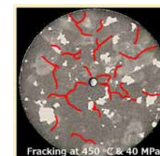
Fig.5 Supercritical hydraulic fracturing in ductile granite
