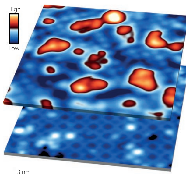
Scanning tunneling microscopy images of strontium oxide ( \text{SrO}_x ) islands (red, top) after deposition of SrO on a titanium-oxygen surface (bottom).
