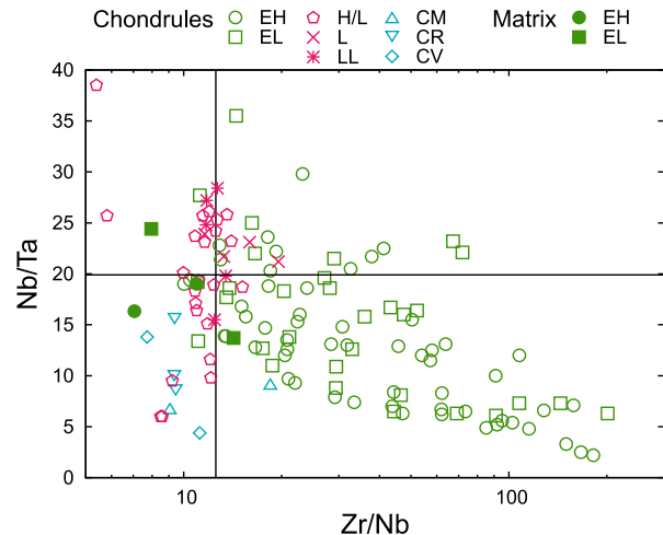
Fig. 1: Nb/Ta vs Zr/Nb of chondrules and matrix. Solid lines represent chondritic values [4, 15].
