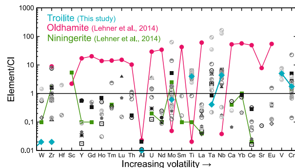
Fig. 2: Mean CI-normalized multi-element pattern of troilites from ECs. Gray plots show data for individual troilite samples. Elements are in order of condensation temperature [19]. Compositions of oldhamite and niningerite from an EH chondrite [11] are also shown.
