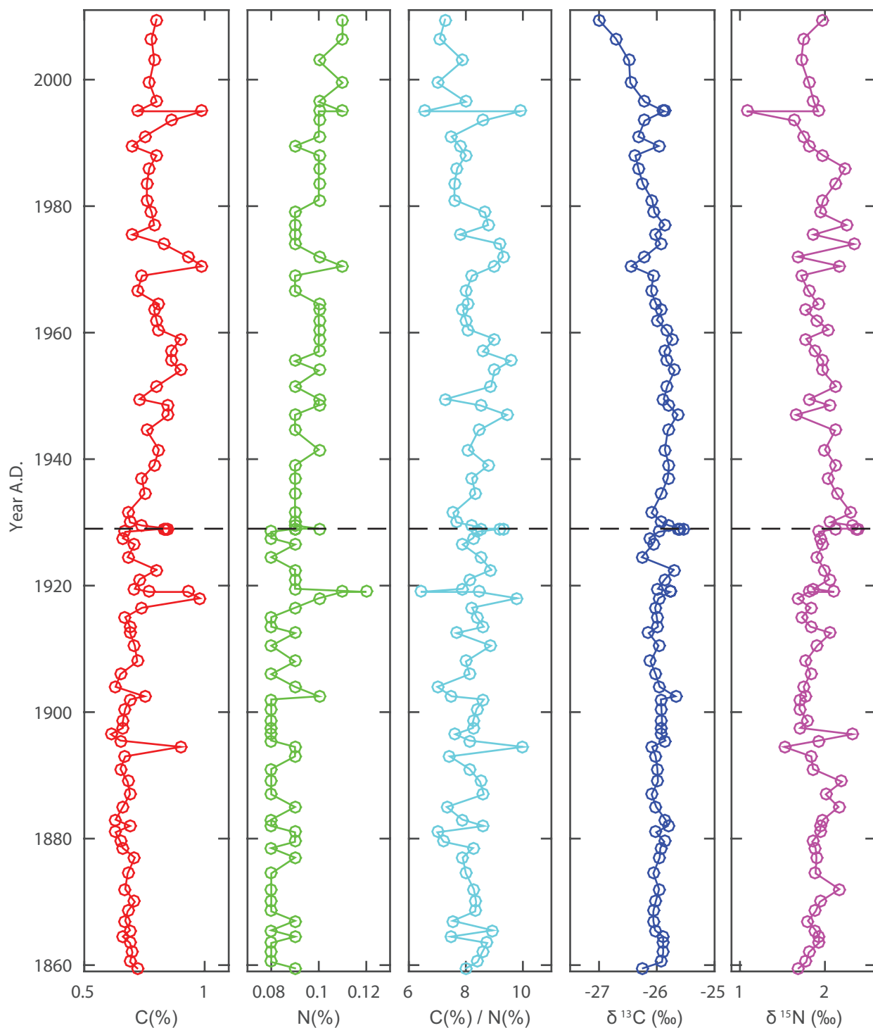
FIG. 5. Geochemical results from core EK 12-01 at Eklutna Lake. Values are plotted against the average year of deposition of each 1 cm 3 sample. The dashed horizontal line emphasizes the date (1929) when the first dam was installed on the Eklutna River.
