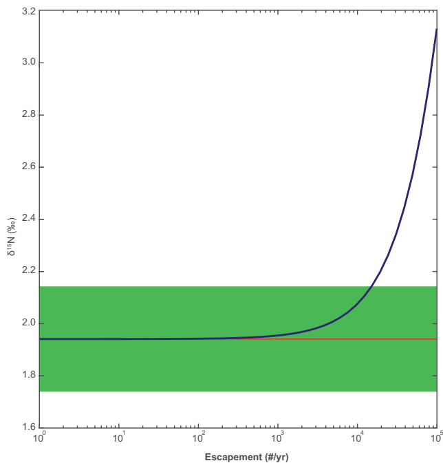
FIG. 7. Results of a sensitivity test predicting the impact of salmon escapement on the nitrogen isotopic composition of the lakebed at Eklutna Lake. The dark blue line shows the isotopic composition expected on the basis of salmon numbers; note that the x-axis is logarithmic. A non-linear relationship between escapement and \delta^{15}\text{N} is expected from the mixing relationship (Finney, 1998; Schindler et al., 2005). The red horizontal line represents the average nitrogen isotopic composition of a completely non-anadromous system, where the width of the green bounding box reflects both the instrumental uncertainty and the observed natural variability around that mean.
