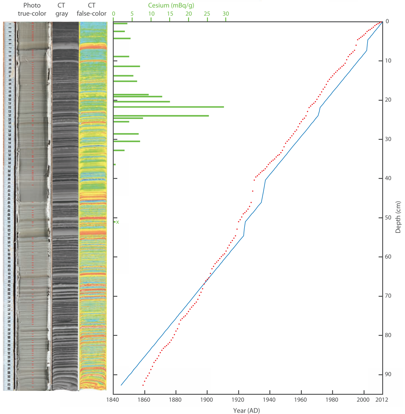
FIG. 3. Age model results for core EK 12-01. At left (L to R), vertical bars show a true-color photo and gray-scale and false-color CT scans of the split core. Boundaries between laminations are marked with faint red lines on the photo. At right, plot shows ^{137}\text{Cs} activity (green) and age models based upon varves (red dots) and ^{210}\text{Pb} (blue line). ^{137}\text{Cs} activity (green bars measured on x-axis at top of plot) includes a short bar at 52 cm depth, marked with an “x,” which denotes a measurement with undetectable ^{137}\text{Cs} activity. The varve-based age model shows the inferred year of deposition (x-axis at bottom of plot) plotted on the average depth of each lamination. The ^{210}\text{Pb} -based age model reflects the estimated average sedimentation rate, with hiatuses (steps in the line) at four discrete high-sedimentation rate events.
