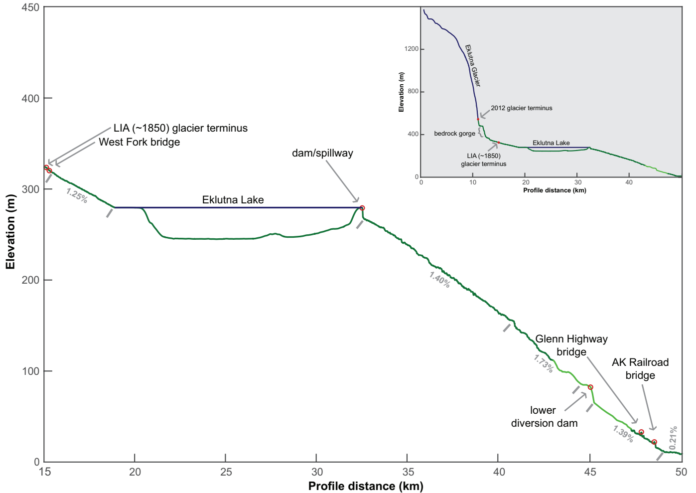
FIG. 2. Profile of Eklutna River and Lake showing select points of interest (red circles). Light gray bars below the profile bracket the reaches of the river over which average stream gradients were calculated. The portion of the profile in light green, near the lower diversion dam, denotes a section in which the profile was smoothed to remove noise generated by errors in the digital elevation model. Inset panel shows the same profile with the Eklutna Glacier (up to its head at Whiteout Pass) for context.
