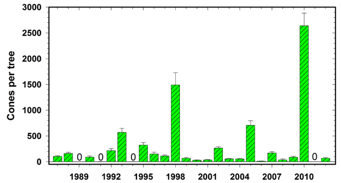
FIG. 11. White spruce cone counts in the Kluane area, 1986 to 2011. Cone counts are carried out on an average of 700 trees each year. Counts were corrected to be whole tree estimates using the method of LaMontagne et al. (2005). Error bars are 95% confidence limits. (Modified from Krebs et al., 2012.)
