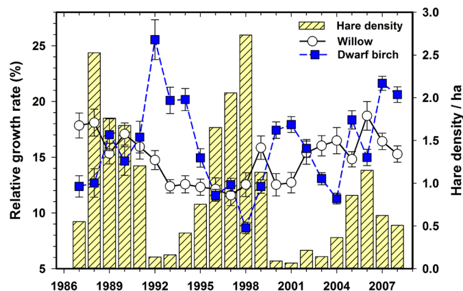
FIG. 12. Relative growth rates of 5 mm diameter twigs of grey willow and dwarf birch at Kluane, 1987 to 2008. Error bars are 95% confidence limits. (C. Krebs, unpubl. data.)
