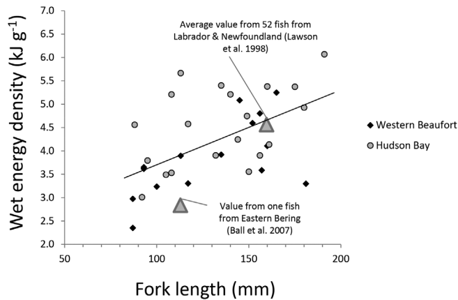
FIG. 3. Relationship between fork length (mm) and at-colony wet energy density ( \text{kJ g}^{-1} ) with data from both sites (parameter SE in parentheses). Wet \text{ED}_{\text{kJ/g}} = 0.015 (\pm 0.0004) \cdot \text{Fork Length}_{\text{mm}} + 2.25 (\pm 0.58) . Mean values from fish sampled in two other studies with similar conditions are also plotted on this graph ( \Delta ) to show general concordance.
