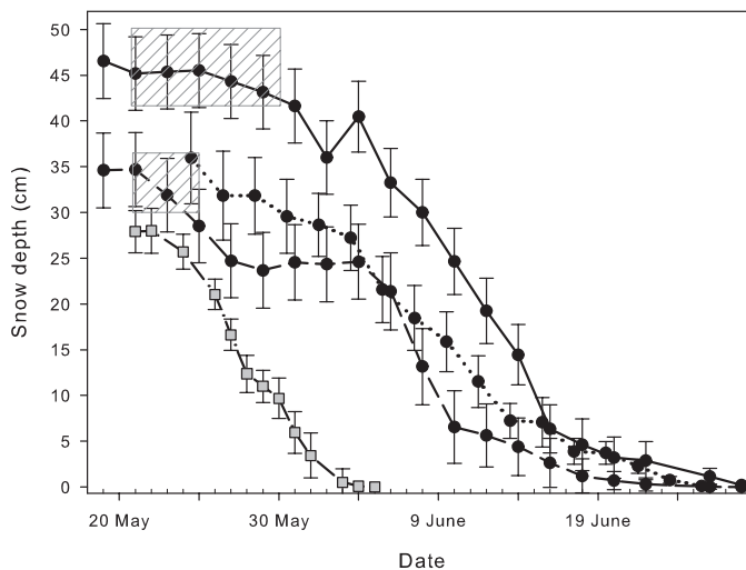
FIG. 2. Change in snow depth along transects during snowmelt on Herschel Island in spring 2009 (gray boxes, dashed-dotted line) and on Bylot Island (black circles) in spring 2010 (solid line), spring 2011 (dashed line), and the long-term mean for 1995–2011 (dotted line). Error bars represent SE. Hatched areas represent periods when trapping took place on Bylot Island each year.
