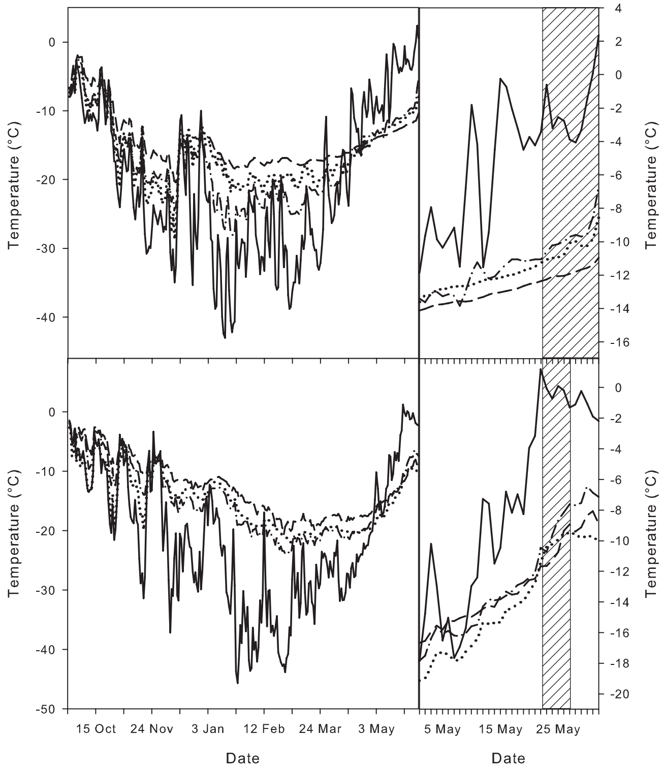
FIG. 3. Comparison of daily temperatures on Bylot Island during winters 2009–10 (upper panel) and 2010–11 (lower panel). Lines show temperatures of ambient air (solid line), subnivean space with 60 cm or more of snow cover (dashed line), subnivean space with less than 60 cm of snow cover (dashed-dotted line), and trapping boxes (dotted line). Hatched areas represent periods when trapping occurred.
