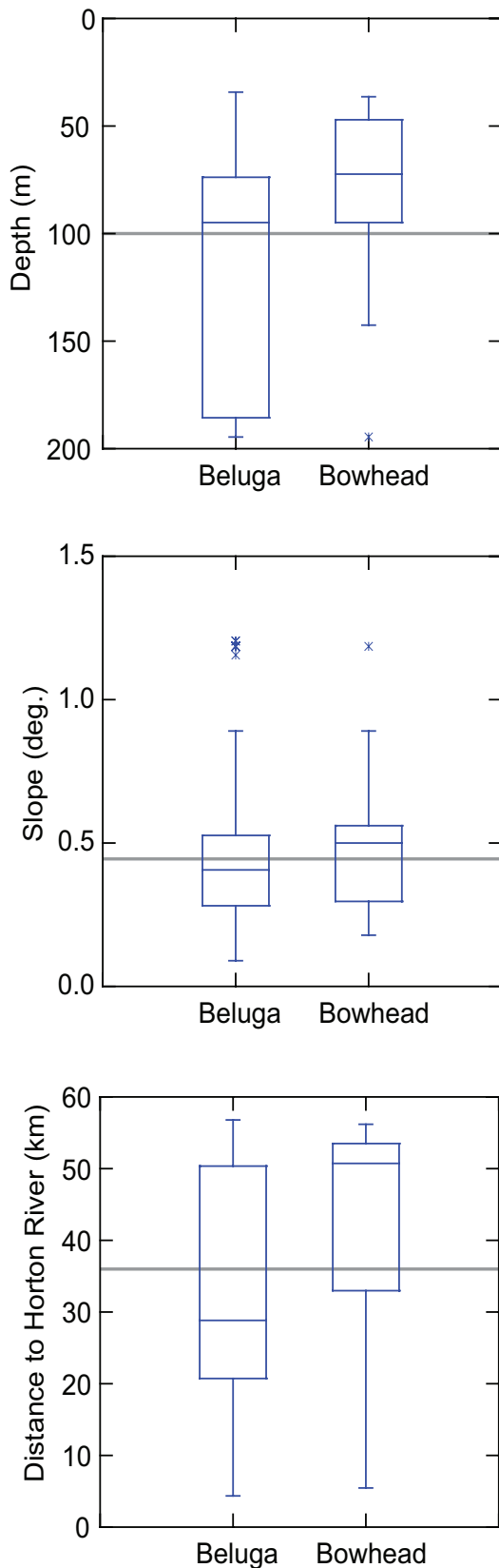
FIG. 6. Box plots of the depth (top), the seafloor slope (middle), and the distance to the Horton River (bottom) for beluga and bowhead sightings. The box encompasses the middle 50% of values, and the line within it indicates the median. The whiskers extend to 1.5 \times the interquartile range and x's indicate near outliers. The grey horizontal line across each plot indicates the average value along the fast-ice edge.
