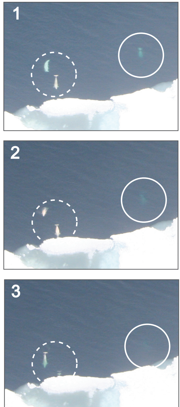
FIG. 4. Examples of shallow dives (dashed circle) and a deep dive (solid circle).
