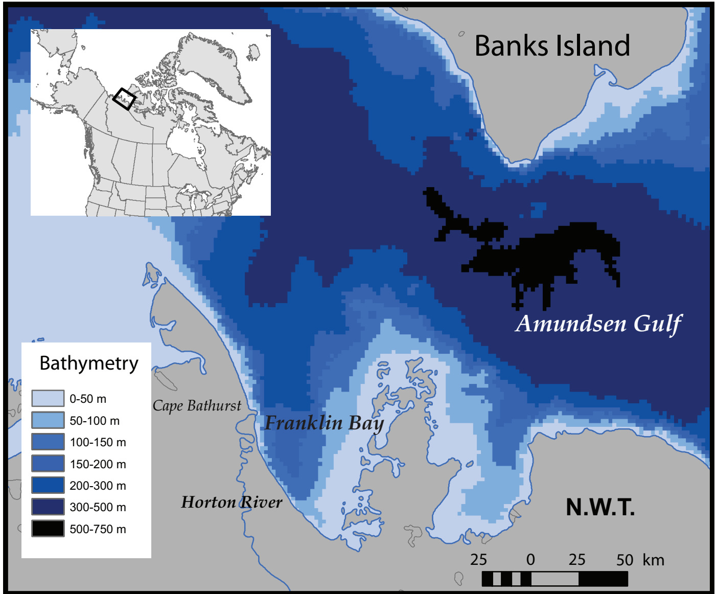
FIG. 1. Study area (bathymetry from Jakobsson et al., 2008).
