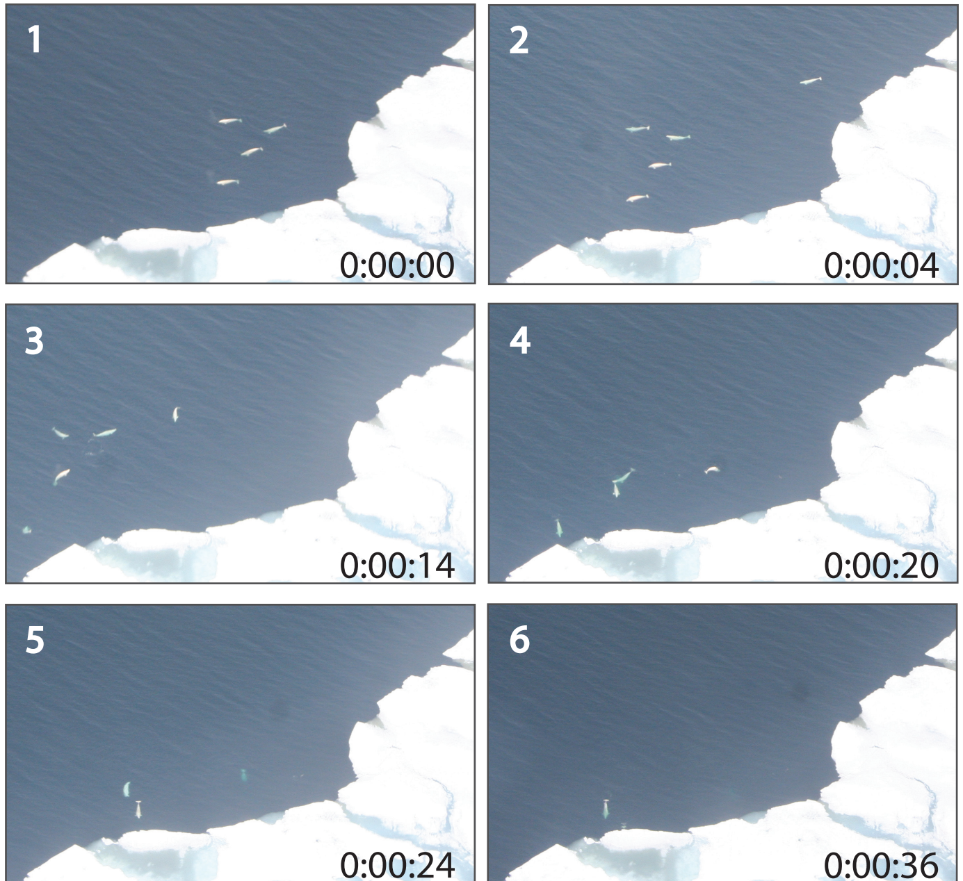
FIG. 5. Sequence of movements of a group of four belugas interacting with a lone beluga. Time stamps indicate elapsed time from image 1 (0:00:00).
