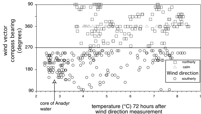
FIG. 4. Seawater temperature at Little Diomed Island in relation to wind vector observed 72 hours earlier at Nome Airport (summer 2001 sampling only). The coldest water temperatures ( < 3.5^{\circ}\text{C} ), which are associated with nutrient-rich Anadyr water, were observed only after southerly winds. Duration and intensity of wind events are not considered in this analysis.
