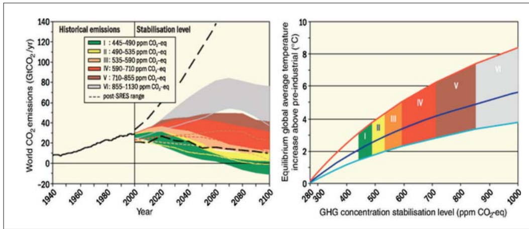
FIGURE 3. CO 2 Emissions and Equilibrium Temperature Increases for a Range of Stabilization Levels 23
