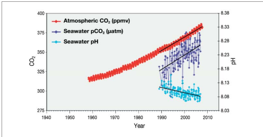
FIGURE A9. CO 2 and pH Time Series in North Pacific Ocean 129
