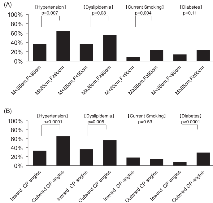
Fig. 3. Prevalence of risk factors between groups
