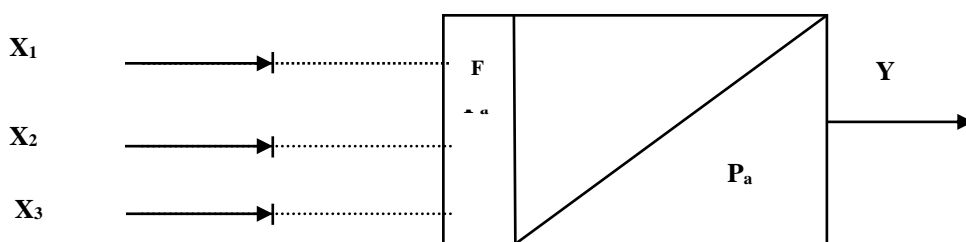
Figure 1.b-The artificial neuron
