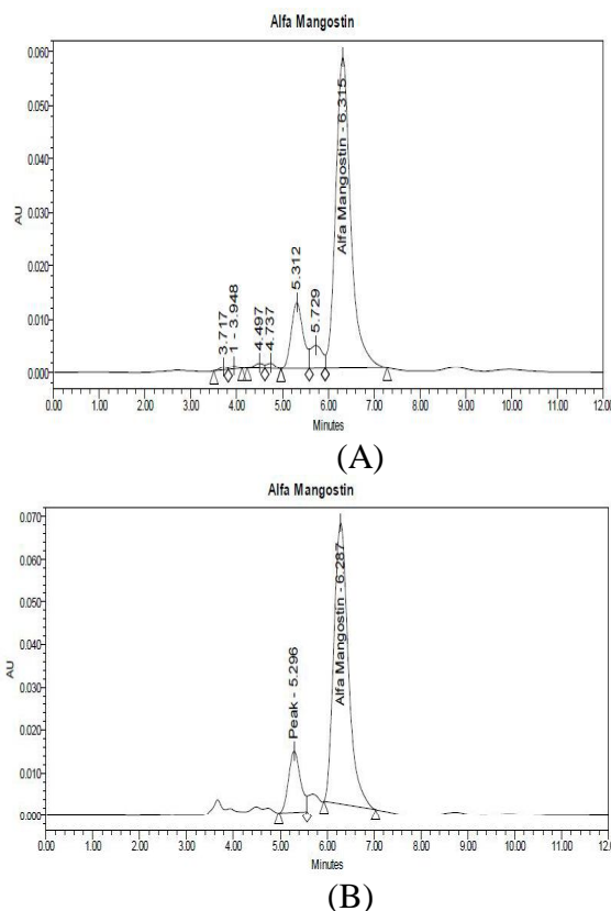
Fig. 4: It shows the typical HPLC chromatograms of \alpha -mangostin under stress condition: thermolysis (A) and oxidation with 3% \text{H}_2\text{O}_2 (B)
