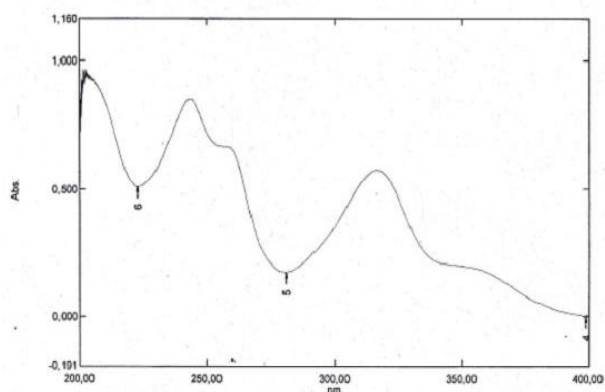
Fig.2 UV absorption spectrum of α-mangostin at a concentration of 10 g/ml in methanol ( \lambda max 243 nm; A:0,854)
