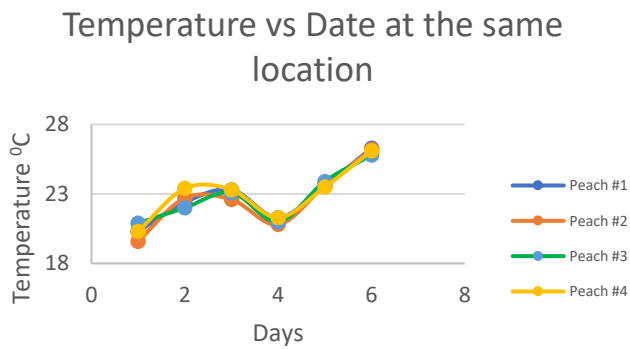
Fig. 3(b) The variation of temperature of peaches at the same location with time
