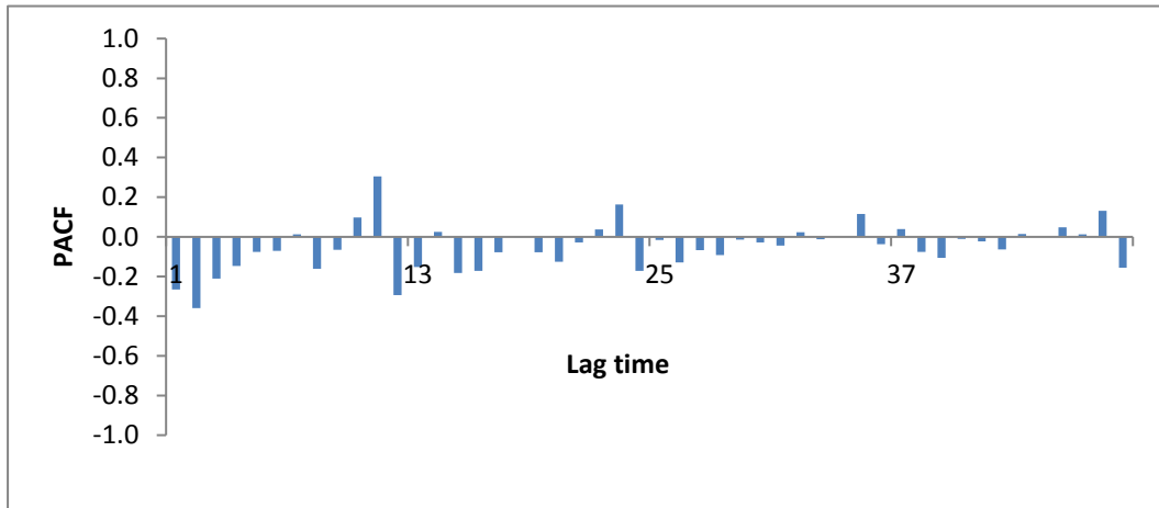
Fig.4: PACF for monthly max temperature with d=1 & D=1
