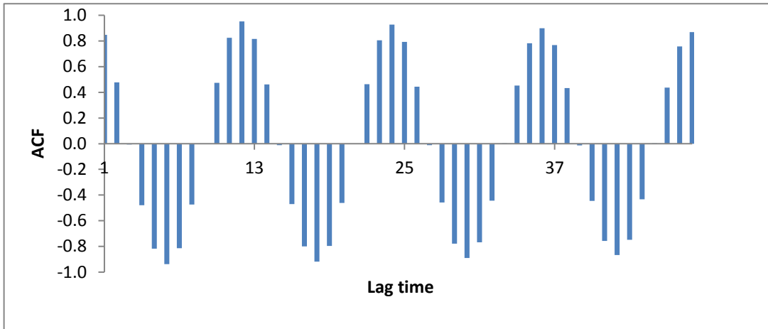
Fig.3: ACF for Max Temperature with d=0 & D=0
