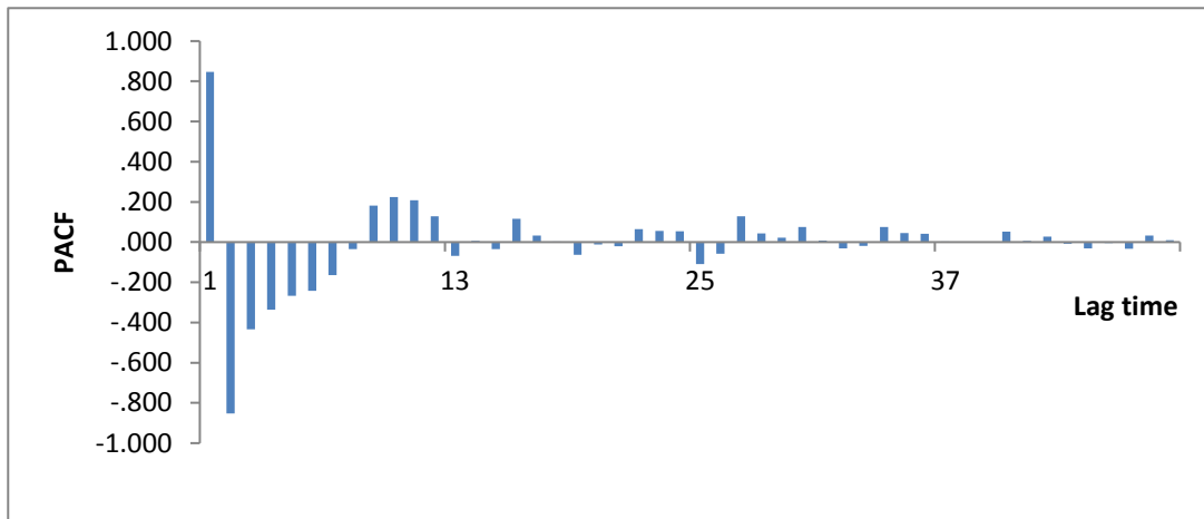
Fig.2: PACF for Max Temperature with d=0 & D=0
