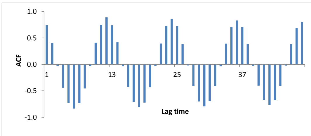
Figure 5: ACF for Max Temperature with d=1 & D=0
