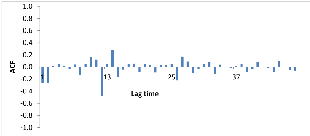
Fig.9: ACF for monthly max temperature with d=1 & D=1
