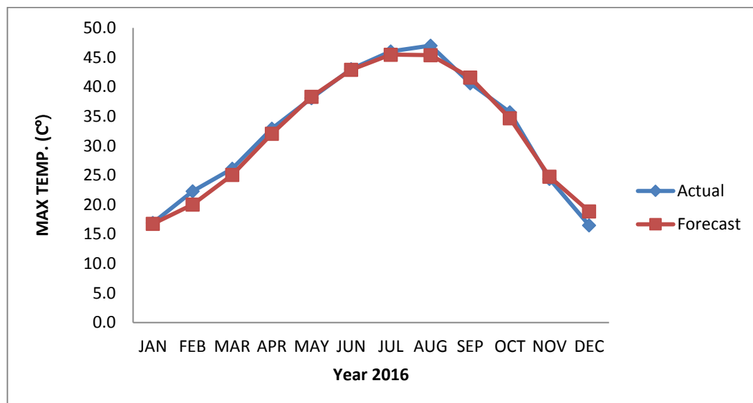
Fig.5: The actual and forecasting monthly max.temperature for the year 2016 using ARIMA (2, 1, 2) × (1, 1, 1) 12 model.
