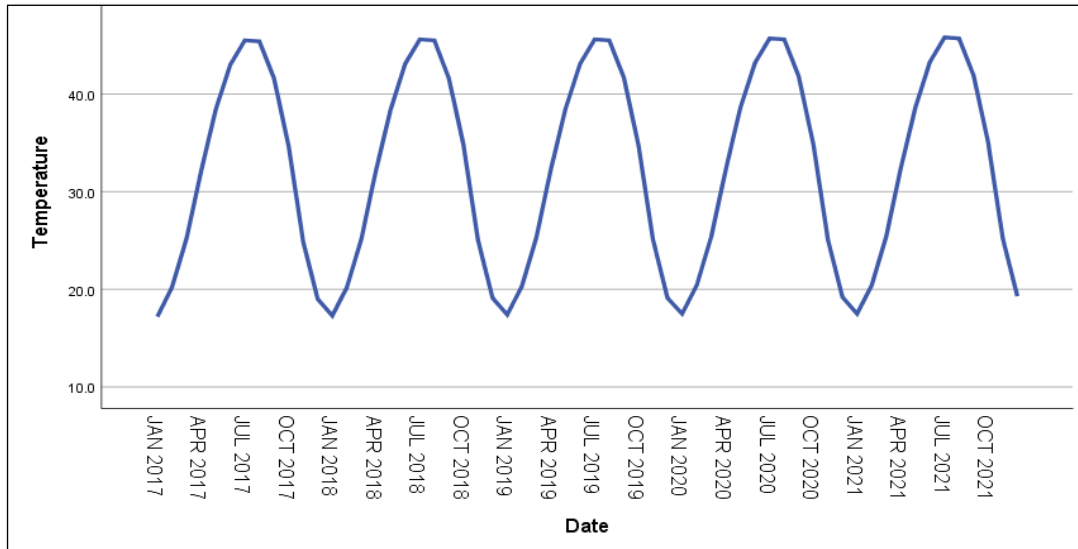
Fig.6: The forecasted time series of max. Monthly temperatures for the period (2017-2021).
