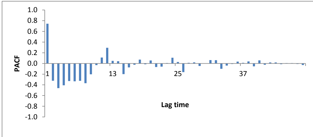
Fig.6: PACF for Max Temperature with d=1 & D=0
