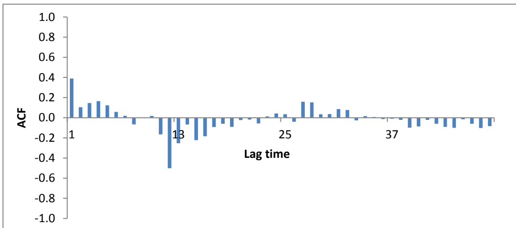
Fig.3: ACF for Max Temperature with d=0 & D=1
