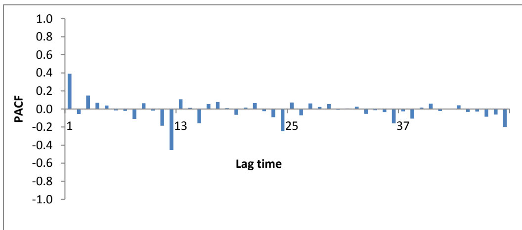
Fig.8: PACF for monthly max temperature with d=0 & D=1
