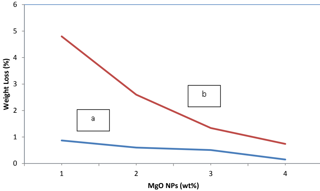
Figure (4): Weight loss as a function of MgO NPs concentration by wear at (a) 15N & (b) 30N
