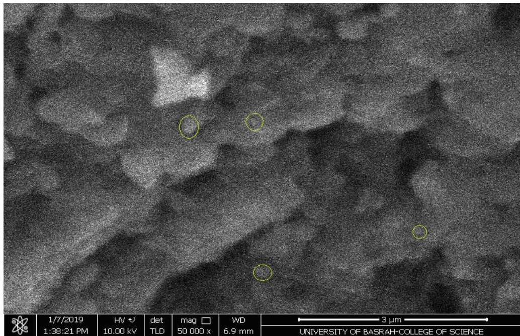
Figure (9): SEM image of composite material SR/MgO NPs at concentration of 9wt%
