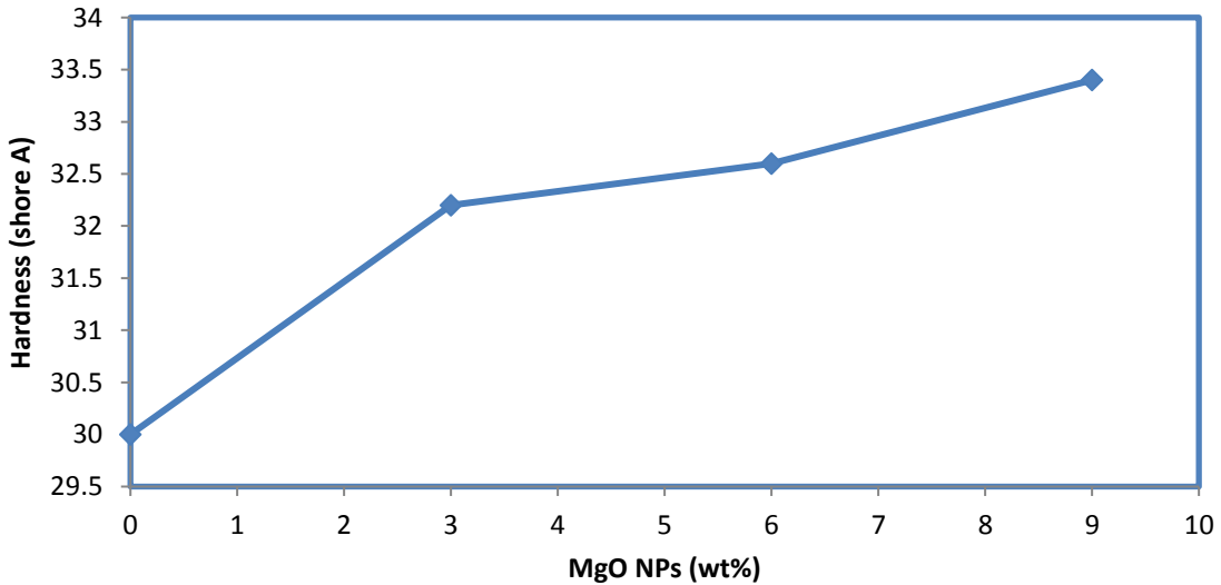
Figure (3): Hardness as a function of MgO NPs concentration
