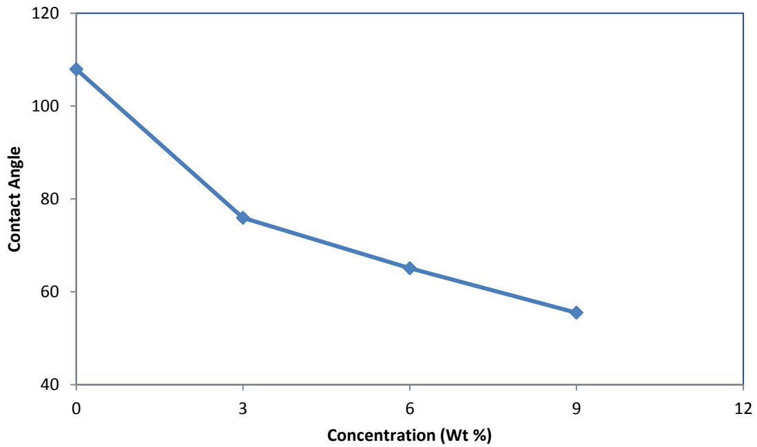
Figure (5): Wettability for SR/MgO NPs
