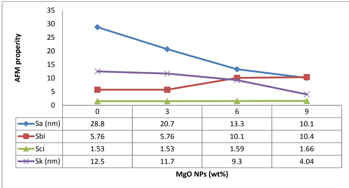
Figure (6): Sa, Sbi, Sci and Sk AFM properties of SR/MgO NPs
