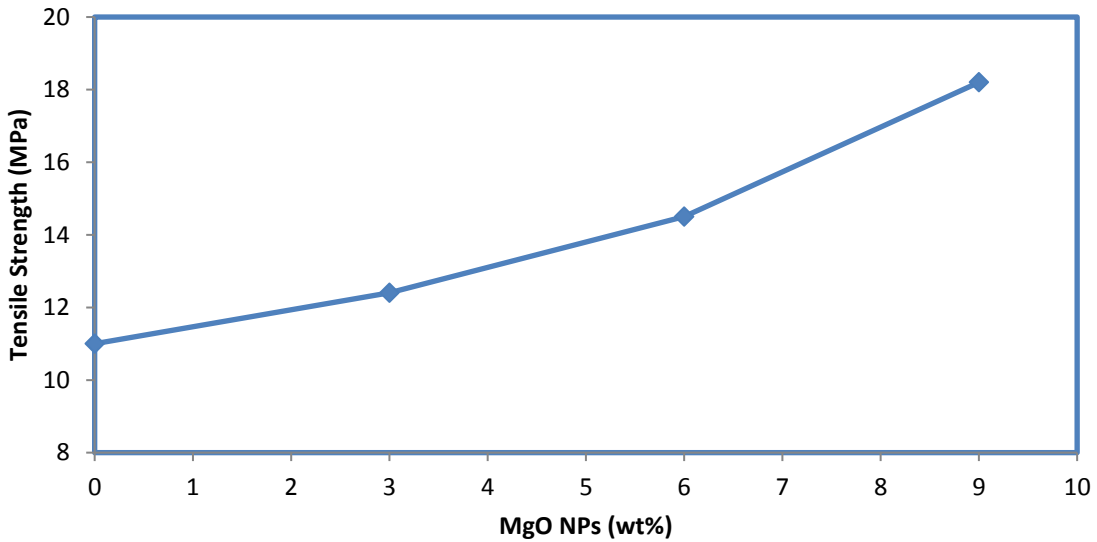
Figure (2): Tensile strength as a function of MgO NPs concentration
