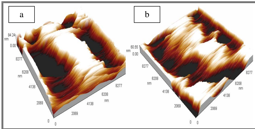
Figure (7): 3D AFM images of (a) SR (b) SR/Mgo NPs (9wt %)
