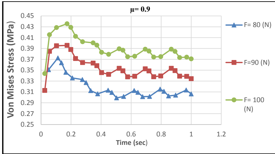
Fig (11) Von Mises stress behavior at \mu=0.9
