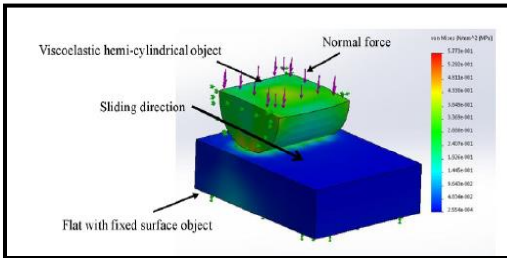
Fig (4): A model of FEA with SOLIDWORKS software.
