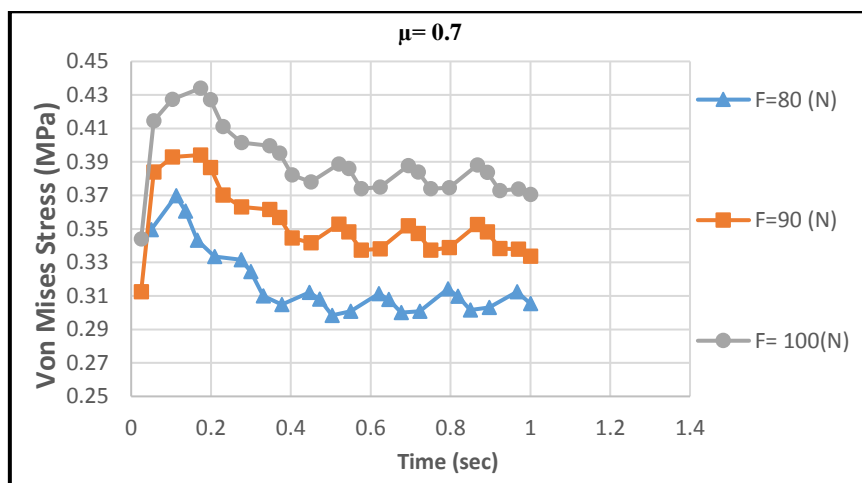
Fig (10) Von Mises stress behavior at \mu=0.7
