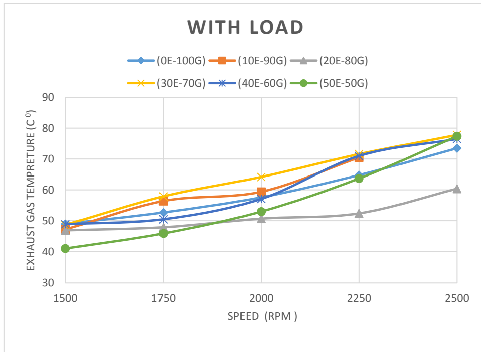
Figure (5): Exhaust gas temperature versus engine speed at different blends
