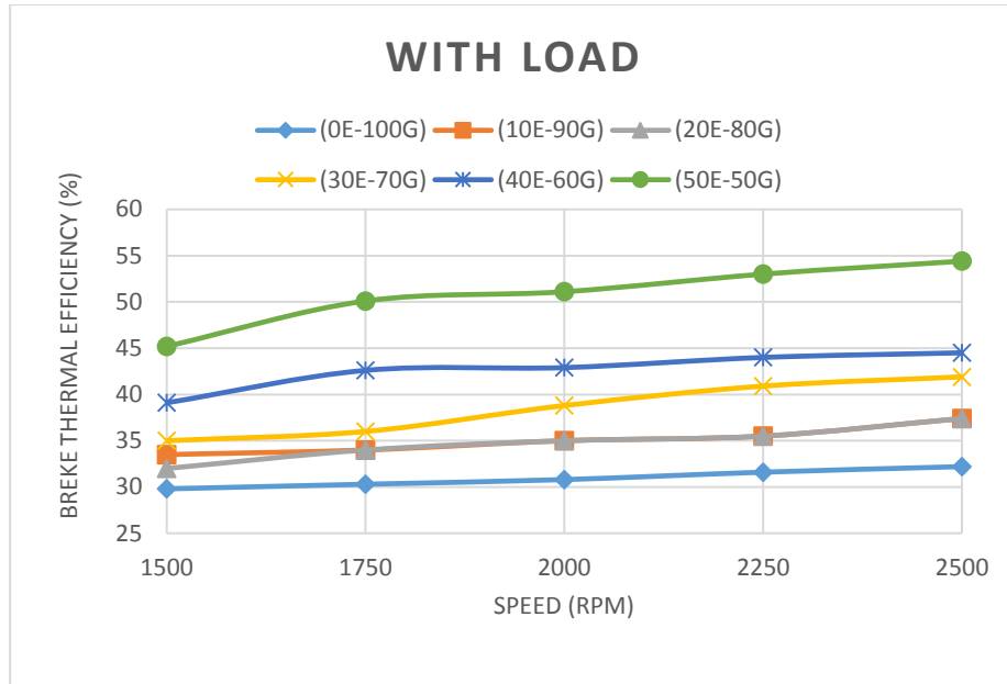
Figure (4): Brake thermal efficiency versus engine speed at different blends
