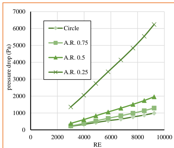
Figure (12): Pressure drop of different tubes aspect ratio with Reynolds number.
