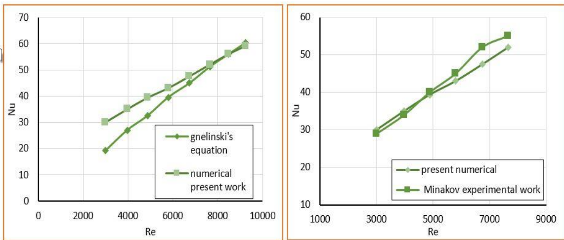
Figure (4): Comparison between numerical average Nusselt numbers with Gnielinski correlation.
