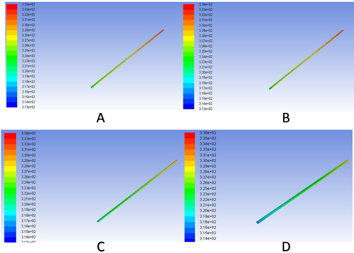
Figure (6): Surface temperature distribution of elliptical tubes with different aspect ratio at Reynolds number 6743 with uniform heat flux: A) Circular tube, B) 0.75 AR, C) 0.5 AR, D) 0.25 AR.
