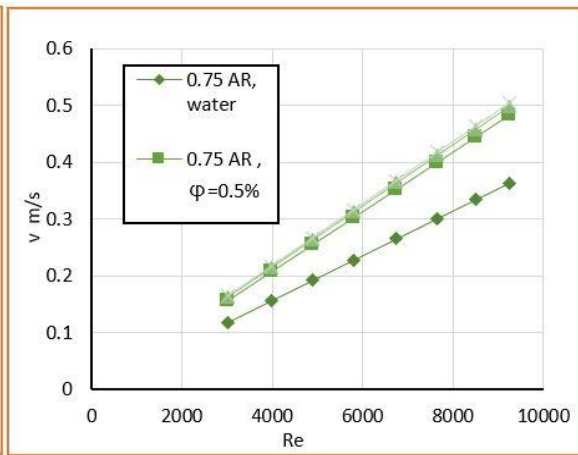
Figure (9): Fluid velocity versus Reynolds number with different nanofluid volume concentrations.
