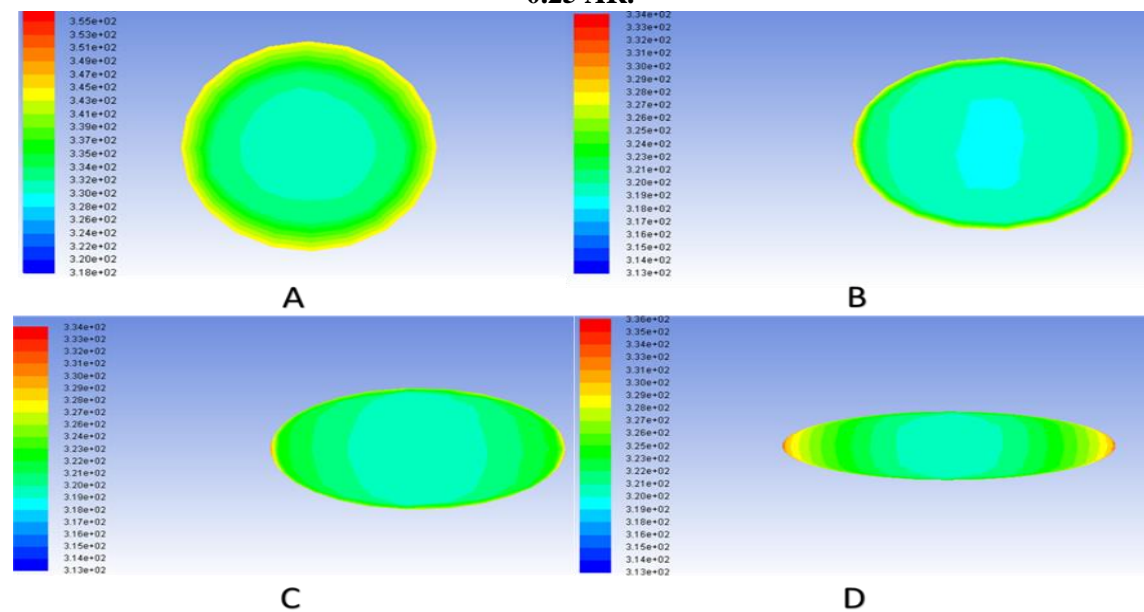
Figure (7): Cross section temperature distribution of elliptical tubes with different aspect ratio at Reynolds number 6743 with uniform heat flux. A) Circular tube, B) 0.75 AR, C) 0.5 AR, D) 0.25 AR
