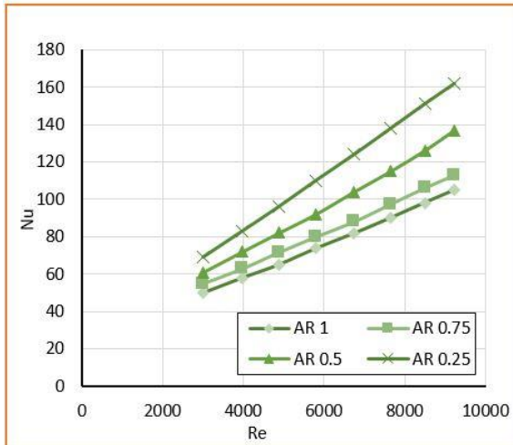
Figure (10): Nusselt number versus Reynolds number at different aspect ratio.
