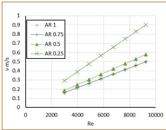
Figure (8): Fluid velocity for different tubes aspect ratio and Reynolds number.
