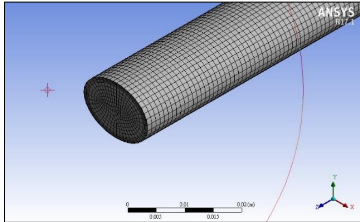
Figure (3): Unstructured used mesh for a 0.75 AR elliptic tube.
