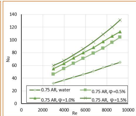
Figure (11): Nusselt number versus Reynolds number at different concentration volume fractions.
