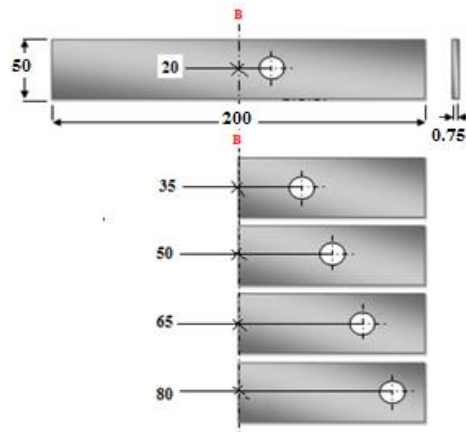
Fig (2): The holes arrangement on sheet metal before bending test.
