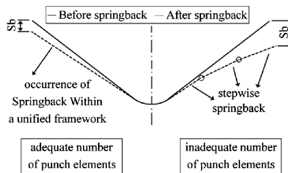
Fig (1): The bent sheet metal before and after springback occurring [9]
