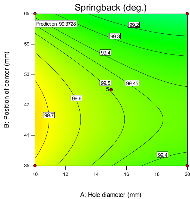
Fig. 7: showing the minimum springback for hole diameter 10 mm and hole location 65 mm for 12 mm depth
