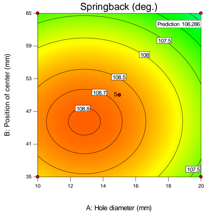
Fig. 6: Minimum springback for hole diameter 20 mm and hole location 65 mm for 12 mm depth
