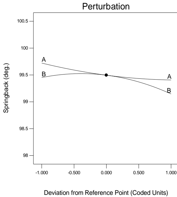
Fig.5: Showing the effect of each parameter on springback for 19 mm depth
