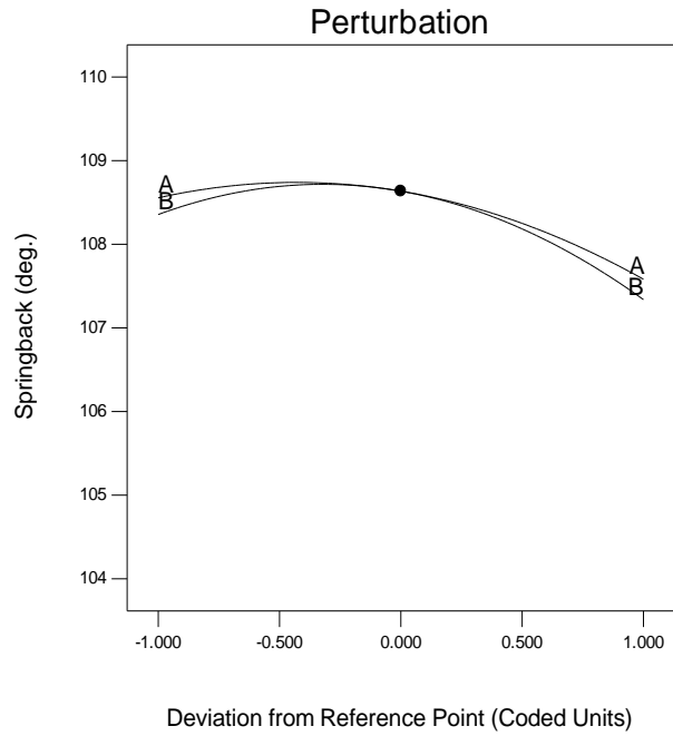
Fig. 4: Showing the effect of each parameter on springback for 12mm depth
