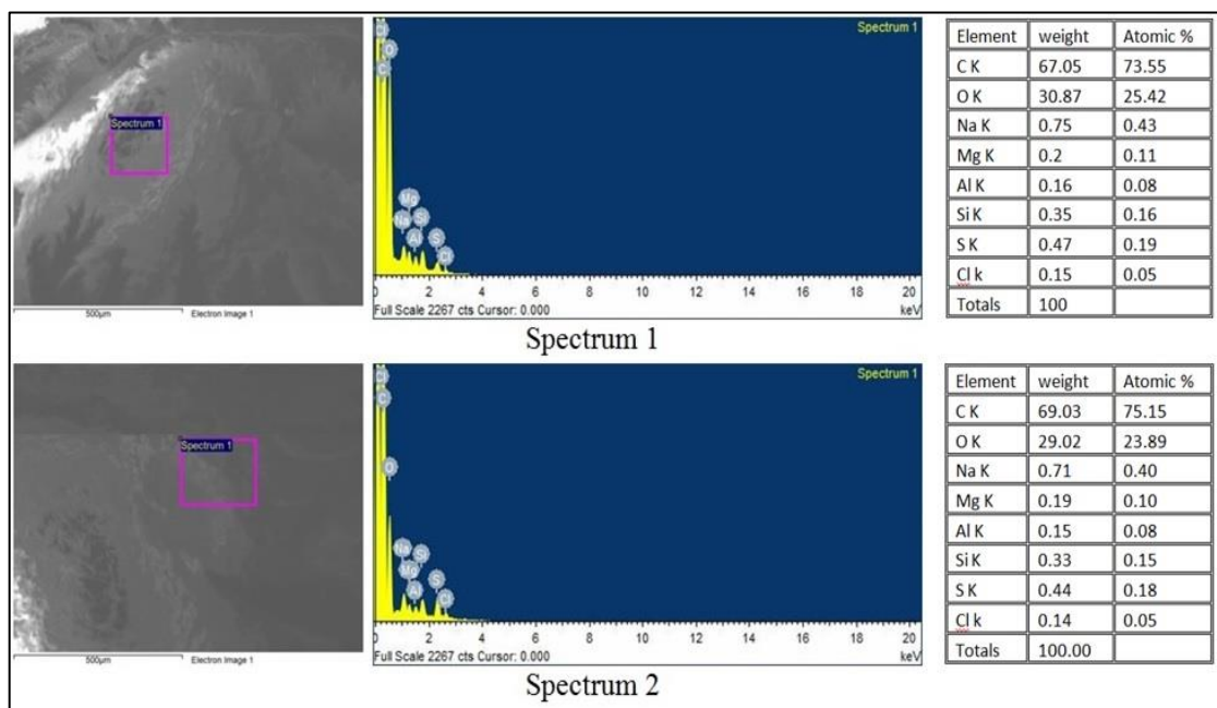
Figure 12. Elementary analysis for hard grade (modified) bitumen
