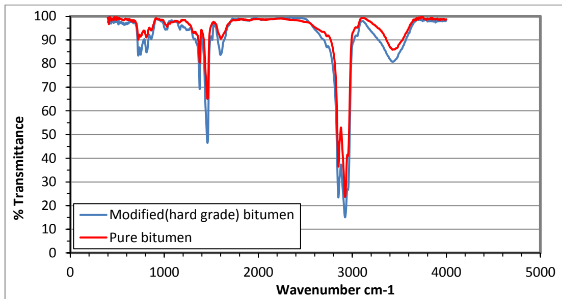
Figure 10. FTIR test results for pure and hard grade bitumen
