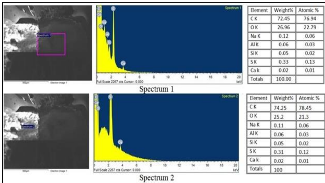
Figure 11. Elementary analysis for conventional 40-50 (unmodified) bitumen
