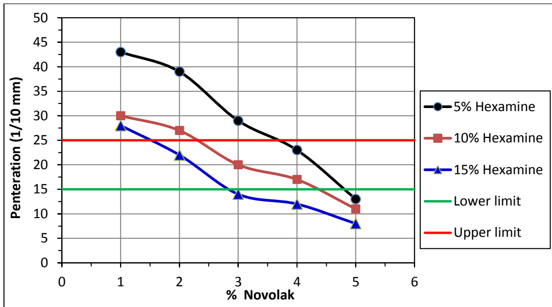
Figure 7. Penetration of bitumen has different ratios of Novolac and Hexamine [22].
