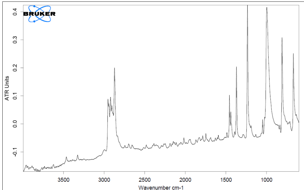
Figure 6. FTIR test results of Hexamine
