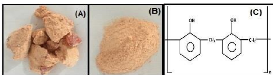
Figure 1. Novolac (Phenol formaldehyde solid resin) :( A) Novolac particles, (B) Grinded Novolac, (C) Structure of Novolac [20].
