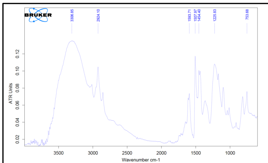
Figure 5. FTIR test results of Novolac
