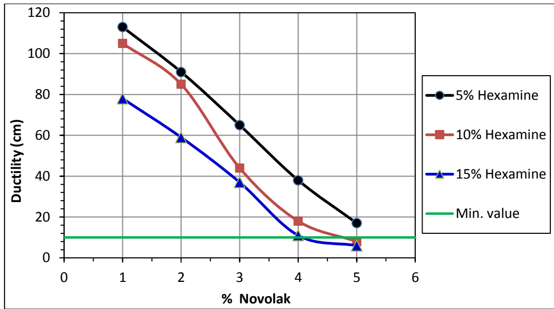
Figure 9. Ductility of bitumen has different ratios of Novolac and Hexamine [6].
