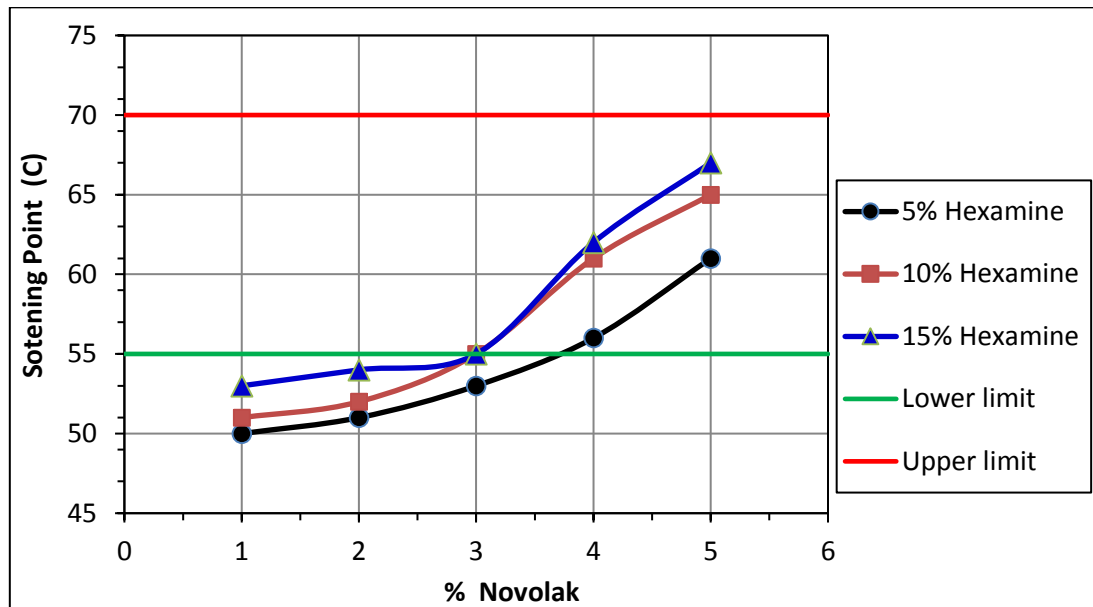
Figure 8. Softening point of bitumen has different ratios of Novolac and Hexamine [22].
