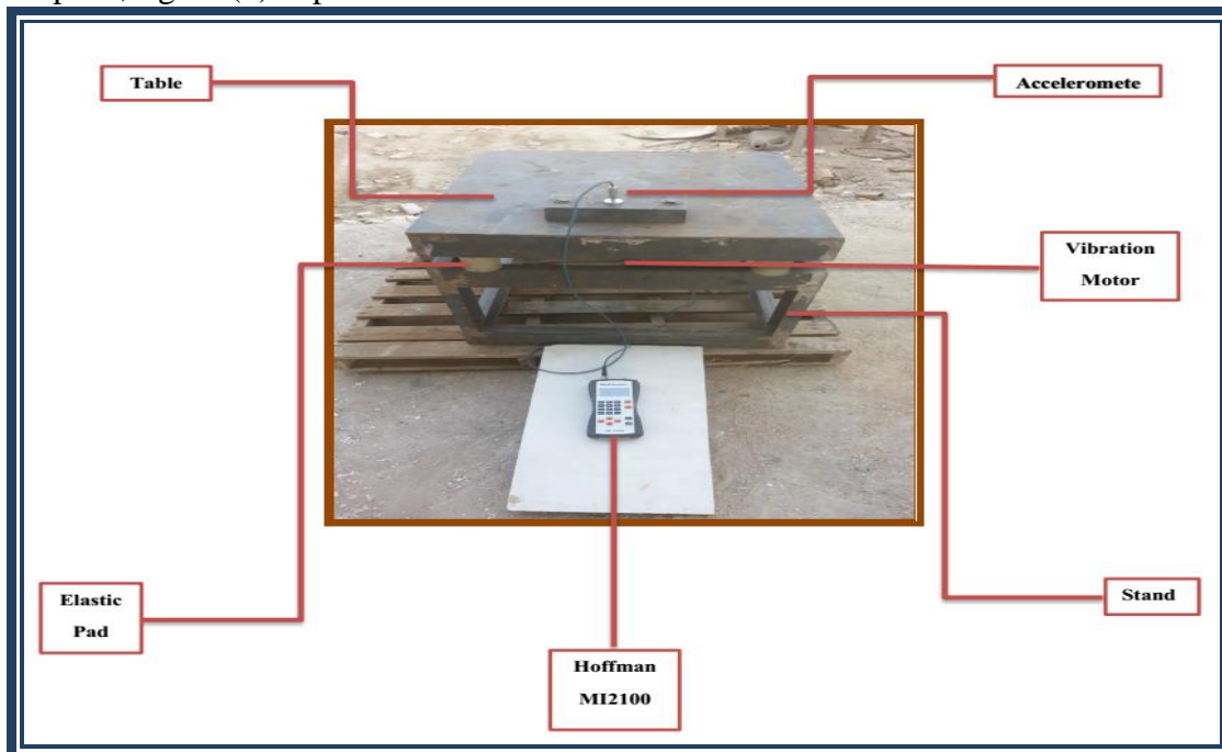
Figure (5) The Vibration Shaker
