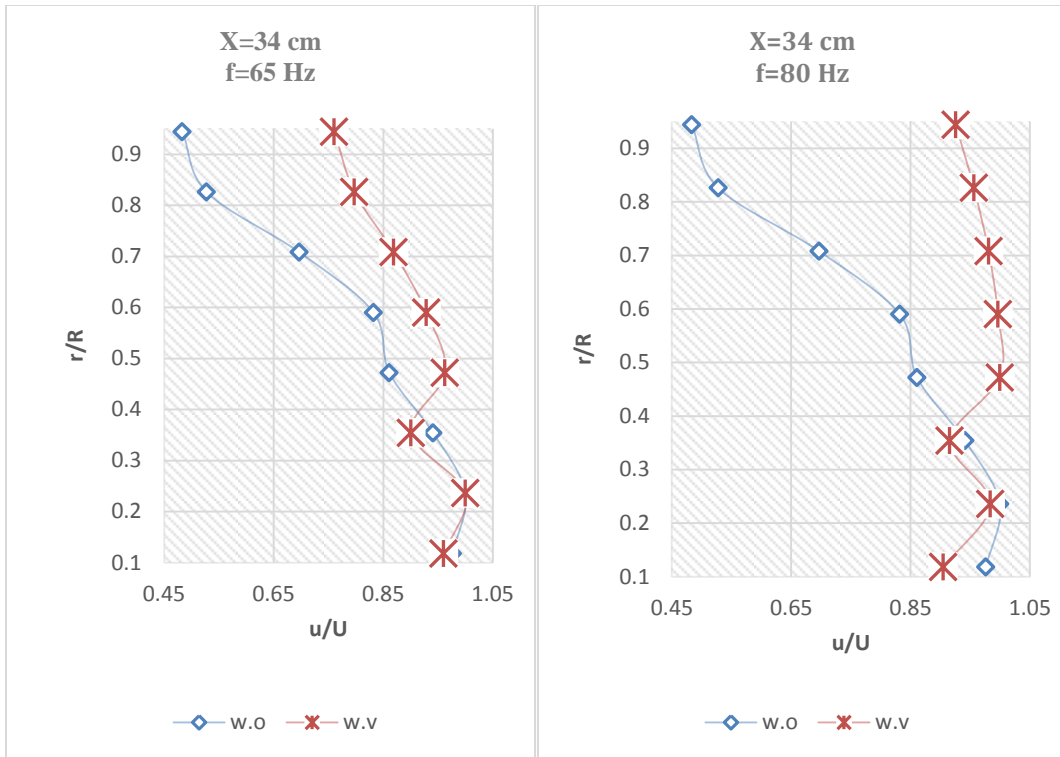
Figure (3):The velocity profile with different frequency at third position (X=34 cm) for upper
