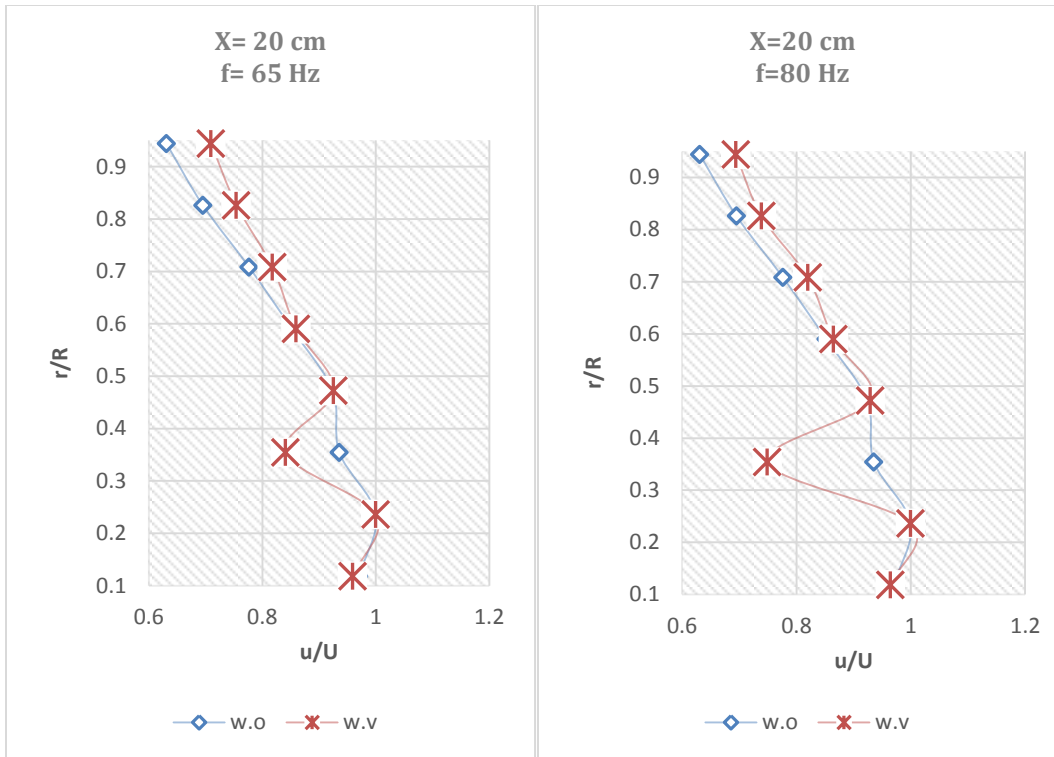
Fig.(2): The velocity profile with different frequency at second position (X=20 cm) for upper
