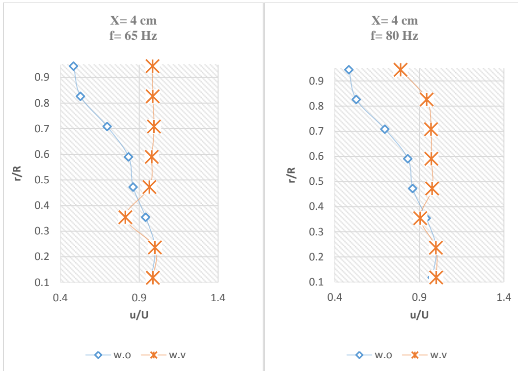
Fig.(1):The velocity profile with different frequency at first position (X= 4 cm) for upper
