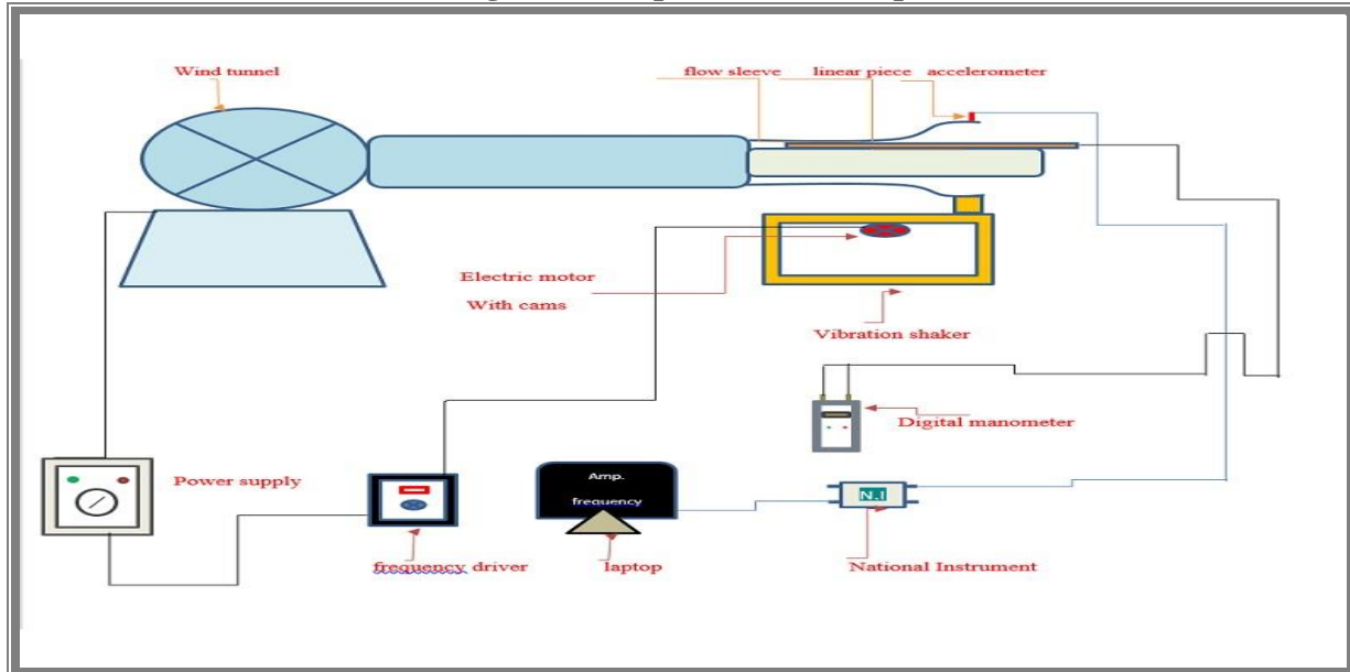
Figure (3) Schematic Diagram
