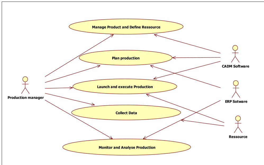
Figure 2: Tha use case diagram of Manufacturing Execution System
