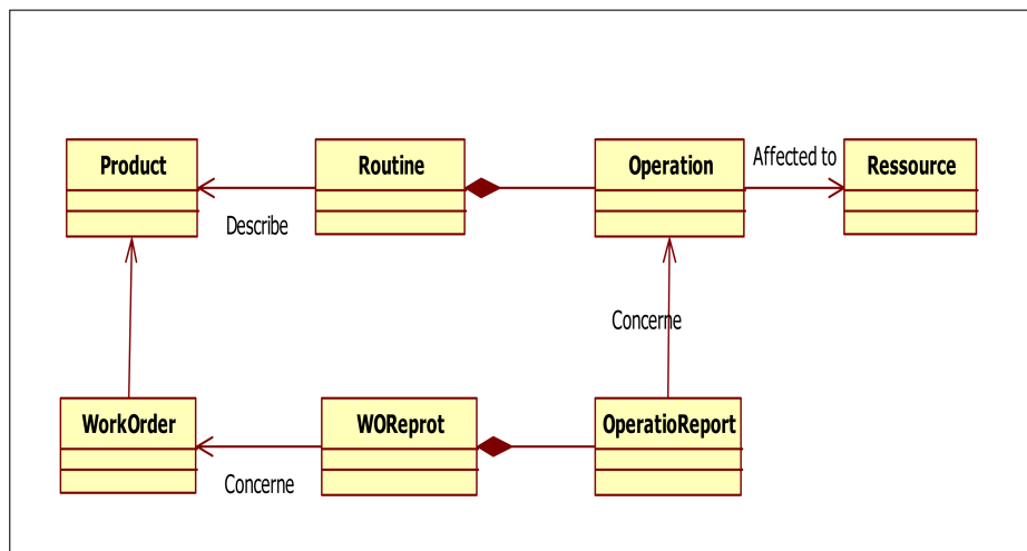
Figure 3: Tha Class diagram of Performance Measurement System
