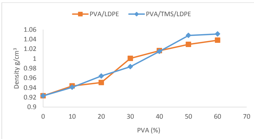
Fig.5: density of PVA/LDPE blend with and without silane.
