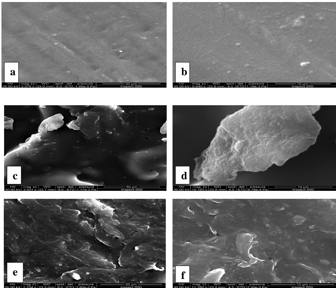
Fig.8: SEM images of pure LDPE (a, b), uncompatibilized polymer blends(c, d) and compatibilized blends (e, f).
