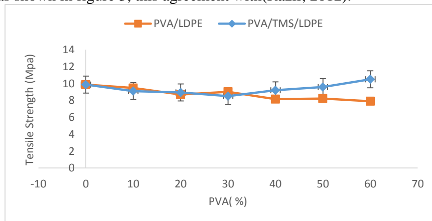
Fig 1: Effect of PVA amount on the tensile strength of PVA/LDPE with and without silane.
