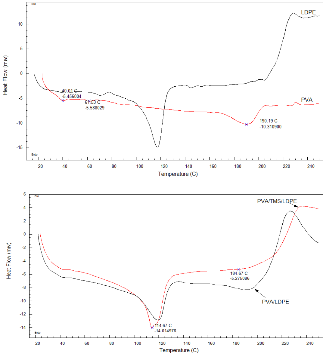
Fig.9: DSC curves for: LDPE, PVA, PVA/LDPE, d)PVA/TMS/LDPE
