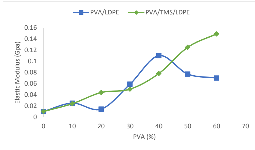
Fig 2: Variation of Young modulus with PVA amount in PVA/LDPE blend with and without silane.
