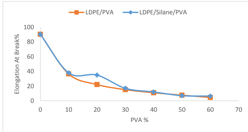
Fig 3: Variation of elongation at break with PVA amount in LDPE/PVA blend with and without silane.
