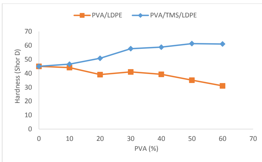
Fig.4: Hardness of PVA/LDPE with and without silane.
