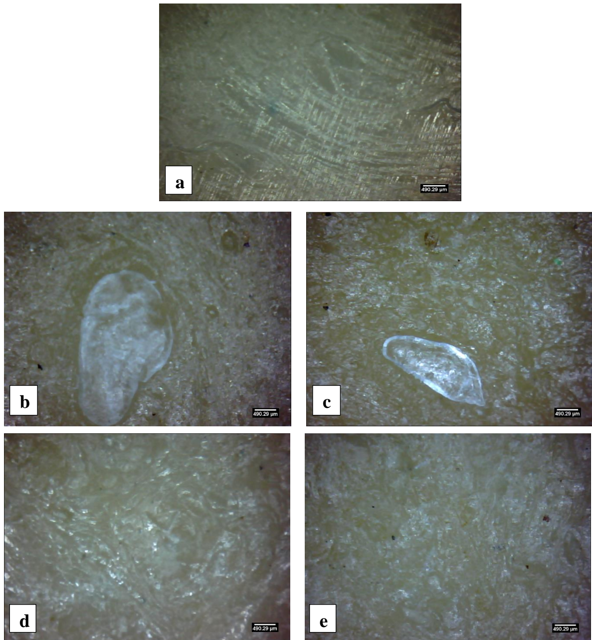
Fig.7: Digital microscope images for: a) pure LDPE, b) 30% PVA + 70% LDPE, c) 40% PVA + 60% LDPE, d) 50% PVA / 5% TMS / 45% LDPE, e) 60% PVA / 5% TMS / 35% LDPE
