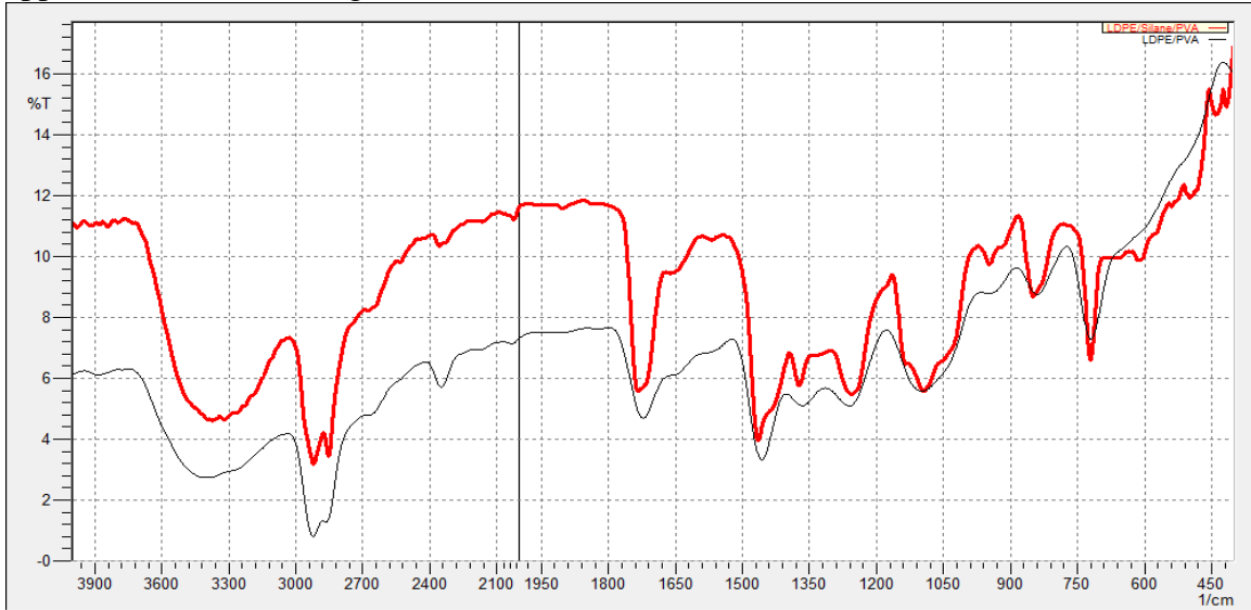
Fig. 6: FTIR spectrum for LDPE, PVA and blend polymers with silane.
