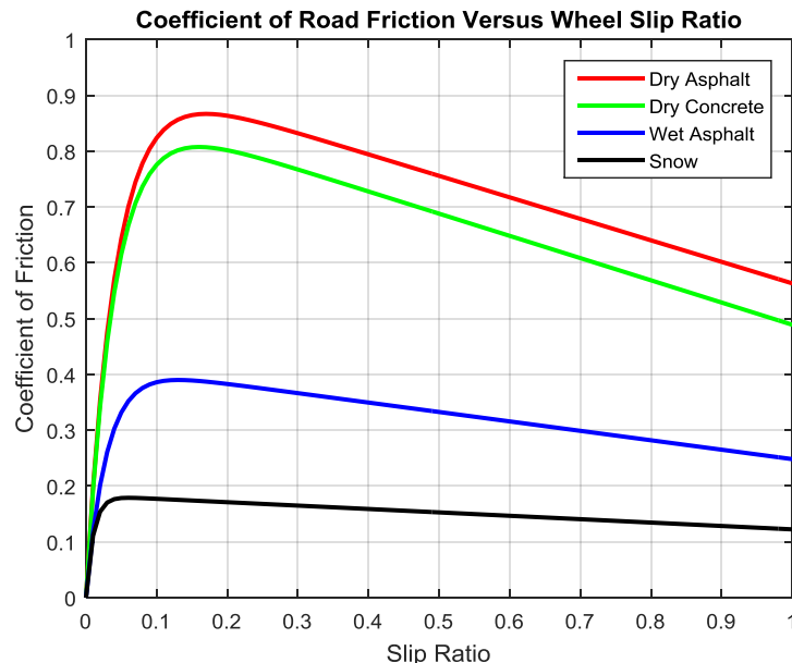
Figure 2: Road coefficient of Frictional VS wheel slip ratio.
