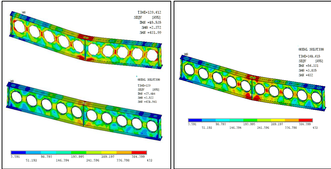
Fig.(16): Stress distribution and deflection of (COOB and COOBR) at failure load of (COOB = 129.0kN ).
