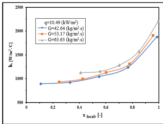
Fig.(6) Effect of mass flux on local heat transfer coefficient at q=10.49 kW/m 2 Fig.(7) Effect of mass flux on local heat transfer coefficient at q=17.17 kW/m 2
