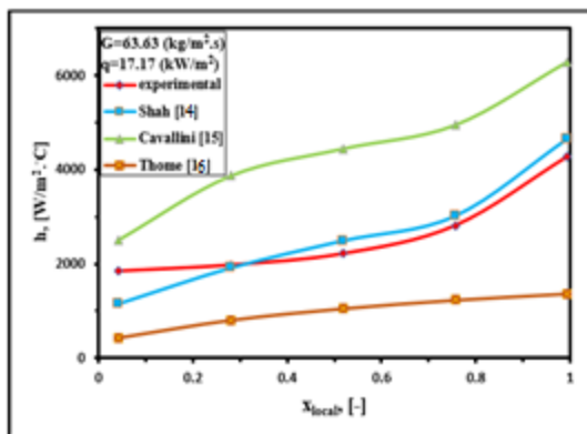
Figure 12. Predicted and experimental heat transfer coefficient as a function of vapor quality for G = 63.63 \text{ kg/m}^2 \cdot \text{s} and q = 17.17 \text{ kW/m}^2 .
