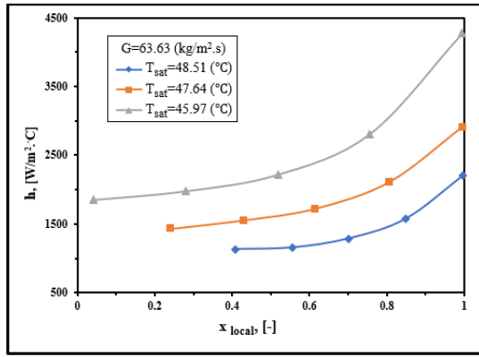
Figure 8. Effect of saturation temperature on local heat transfer coefficient at G = 63.63 \text{ kg/m}^2 \cdot \text{s}
