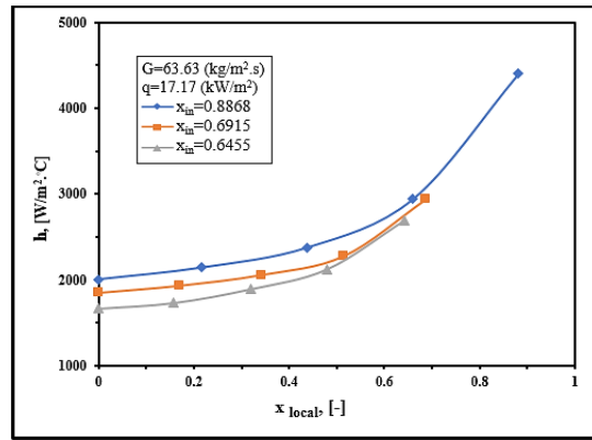
Figure 9. Effect of inlet vapor quality on local heat transfer coefficient at G = 63.63 \text{ kg/m}^2 \cdot \text{s}
