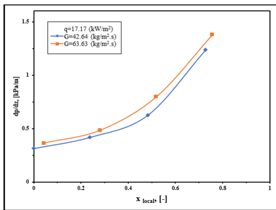
Figure 10. Variation of pressure drop with vapor quality for different mass fluxes and q = 17.17 \text{ kW/m}^2 .
