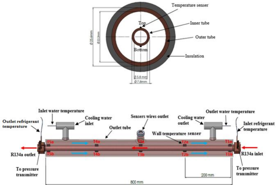
Figure 3. Condenser test section.
