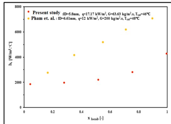
Figure 14. Comparison of present study experimental results with Pham et al. 2015 work.
