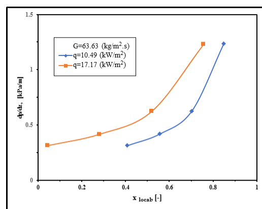
Figure 11. Variation of pressure drop with vapor quality for different heat fluxes and G = 63.63 \text{ kg/m}^2 \cdot \text{s}
