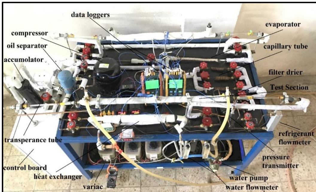
Figure 2. Test rig
