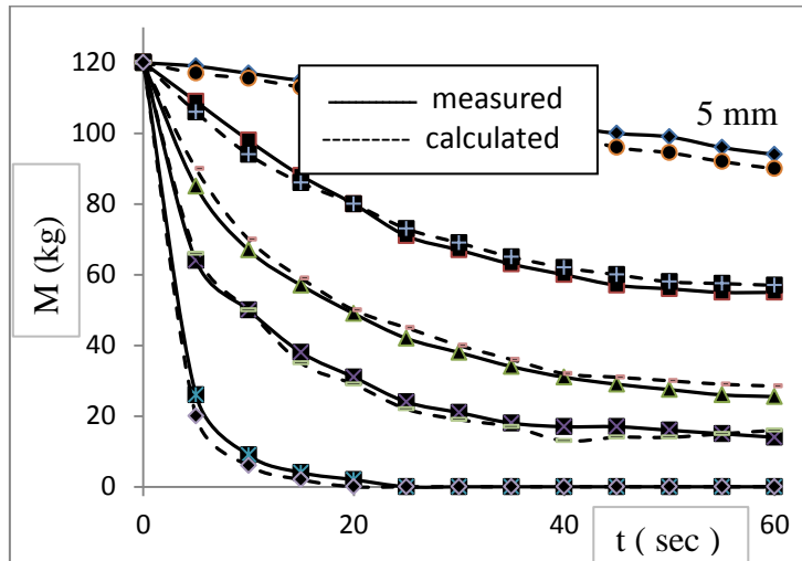
Figure (4): Residual coolant quantity in the vessel for different times (lower pipe with T=558 K^0 )
