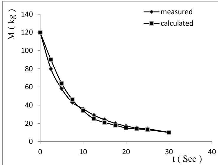
Figure (3): Coolant quantity in the high pressure vessel at different times (leakage hole diameter 32mm, T=558K^0 and P=12.3 MPa for lower leakage)
