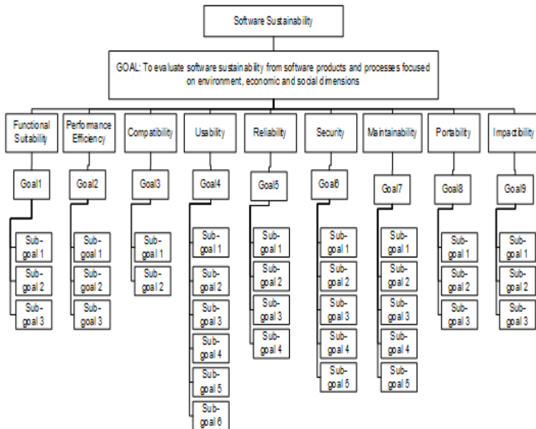
Figure 2. Goal Structure of Software Sustainability Criteria.
