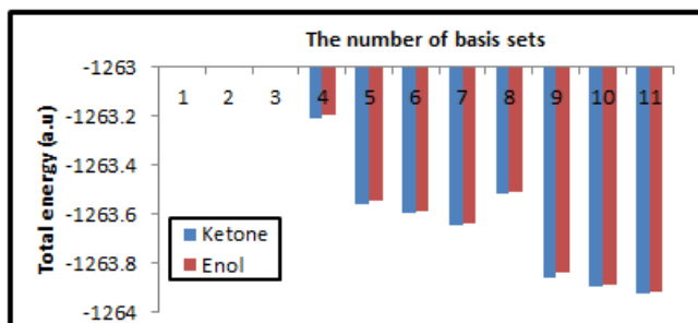
Fig. 3: The total energy of the structures under study as a function of the number of basis sets.
