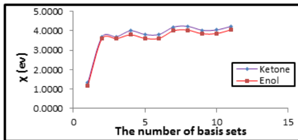
Fig. 10: The electronegativity of structures under study as a function of the number of basis sets.
