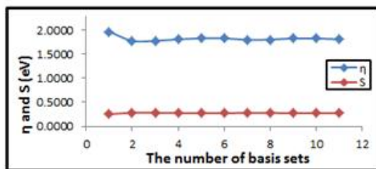
Fig. 8: The chemical hardness and softness of ketone form as a function of the number of basis sets.
