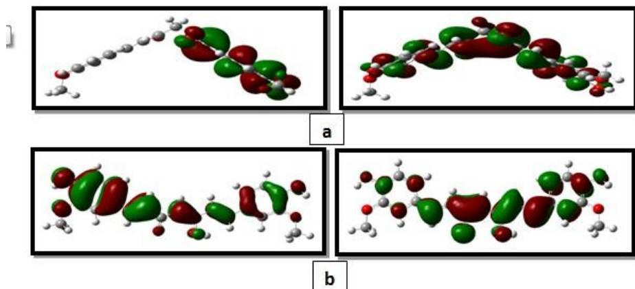
Fig. 5: The distribution of HOMO (left) and LUMO (right) levels for curcumin isomers: a-ketone form and b-enol form.
