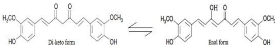
Fig. 1: Structure of curcumin .
