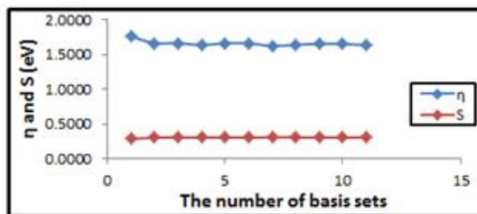
Fig. 9: The chemical hardness and softness of enol form as a function of the number of basis sets.
