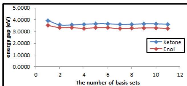
Fig. 4: The energy band gap of two forms, curcumin (ketone) and curcumin (enol), as a function of the number of basis sets.
