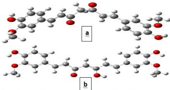
Fig.2: Optimized geometry for curcumin isomers: a- ketone form ( trans ) and b- enol form ( cis ) at the B3LYP/ 6-311+G(d,p) basis set.
