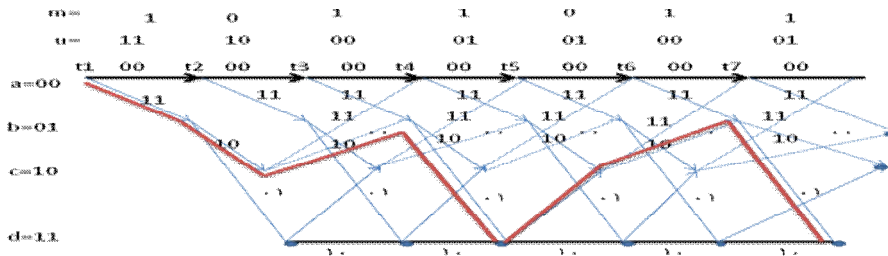
Figure 4. The simulation result of convolutional encoder.
