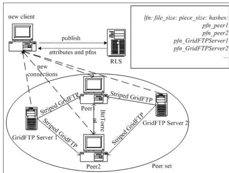
Figure 2: GridTorrent
