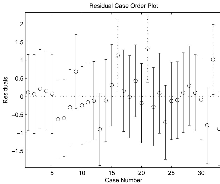
Figure 1: The differences between y_{i_1 \dots i_4} and \ln \frac{P(X_i)}{1-P(X_i)}
