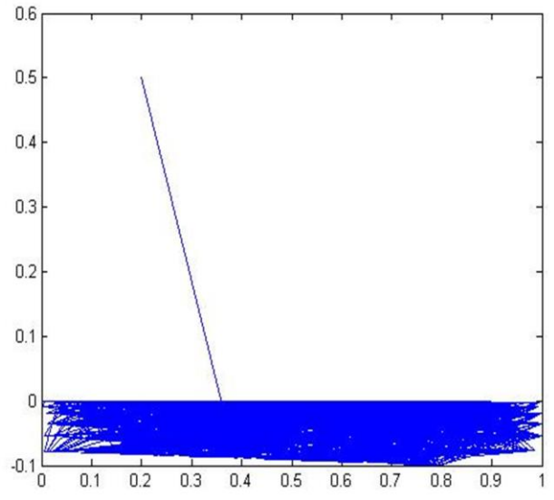
Fig (1-14) \alpha = 3.4 , \beta = -0.1 with initial points (0.1,0.1)
