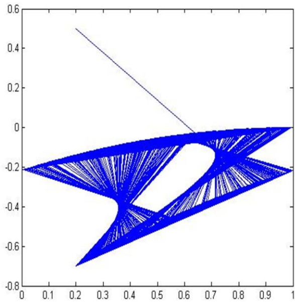
Fig (1-11) \alpha = -0.9 , \beta = -0.7 with initial points (0.1,0.1)
