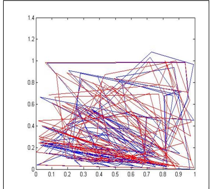
Fig (1-2) \alpha=-3.16 , \beta=0.1 with initial points (0.2,0.1) , (0.4,0.6)
