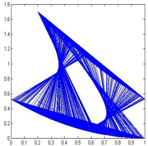
Fig (1-12) \alpha = -0.7 , \beta = 1.7 with initial points (0.1,0.1)
