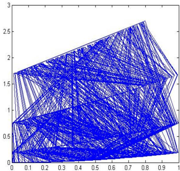
Fig (1-13) \alpha = 1.9 , \beta = 2.7 with initial points (0.1,0.1)
