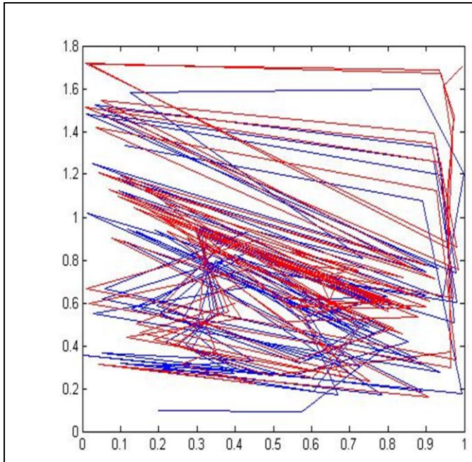
Fig (1-1) \alpha=-1.06 , \beta=0.5 with initial points (0.2,0.1) , (0.4,0.6)
