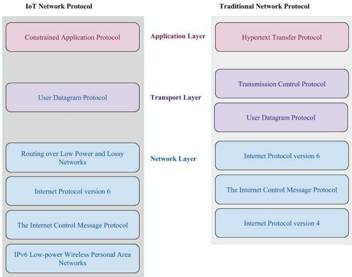
Figure 1: Data Transfer procedures of Internet of Things vs. customary system
