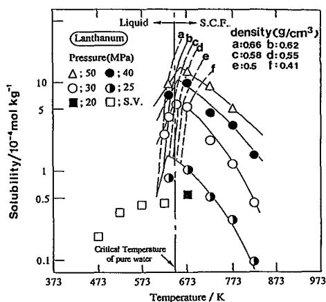
Fig. 1 Isobaric solubility curves for lanthanum compounds in water.
