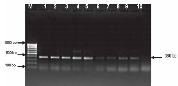
Fig. 3. The amplicons of primers MA1 and MA2 from moderately resistant lines of seedlings tested. M: 100 bp ladder; Lane 1–10: moderately resistant seedlings (05-1103-15, 05-1103-22, 05-1103-14, 05-PR-III-07, 05-992-15, 05-861-04, 05-5271-03, 05-1319-18, 05-1080-01, Negative control)
