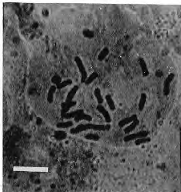
Fig. 1. Metaphase chromosomes of two year-old callus cells of Crocus sativus showing the parental chromosome number 2n=24 (Bar on the figure represents 10 \mu\text{m} )
