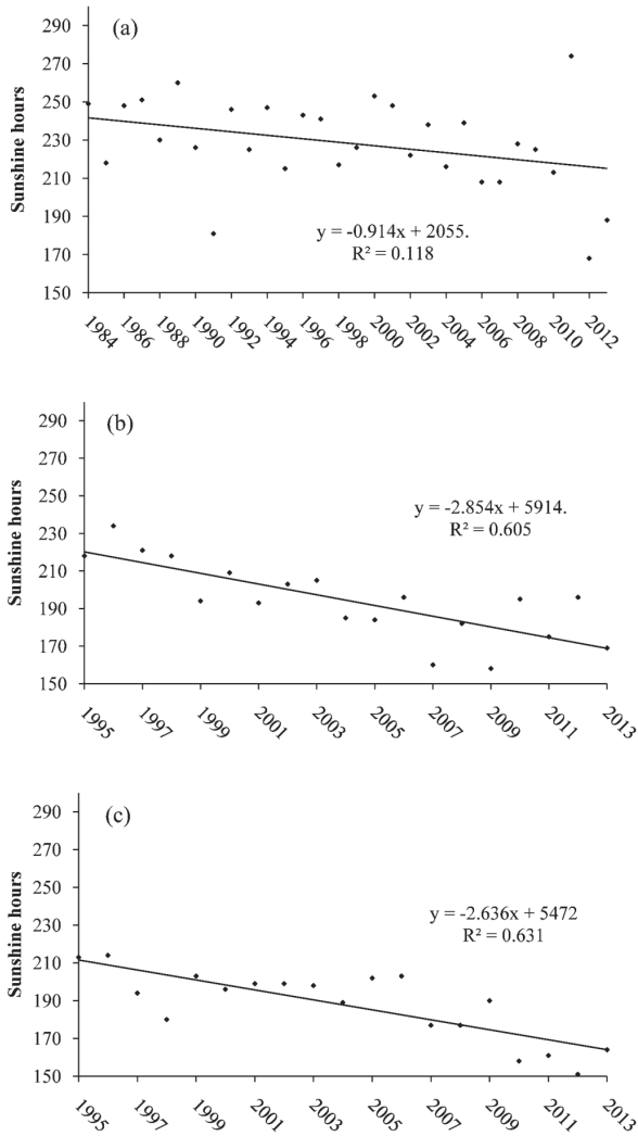
Fig. 1. Annual decreasing trends of daily Bright Sunshine Hours > 5.6 hours for (a)Agartala, (b) Tura and (c) Nagrakata
