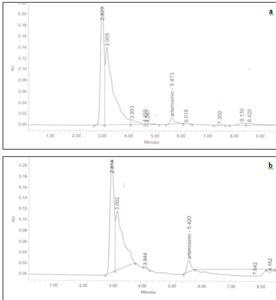
Fig. 6. HPLC chromatogram showing peaks of artemisinin in control (a) and 0.10mM Al treated plants (b) of Artemisia annua L.
