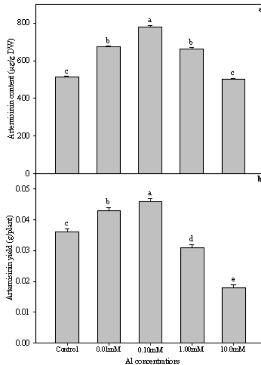
Fig. 5. Effect of different concentrations of Al on artemisinin content (a) and artemisinin yield (b) of Artemisia annua L. Bars showing the same letter are not significantly different at p \leq 0.05 as determined by Duncan's multiple range test. Error bars ( \uparrow ) show SE
