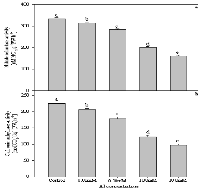
Fig. 2. Effect of different concentrations of Al on NR (a) and CA (b) activities in leaves of Artemisia annua L. Bars showing the same letter are not significantly different at p \leq 0.05 as determined by Duncan's multiple range test. Error bars ( \tau ) show SE
