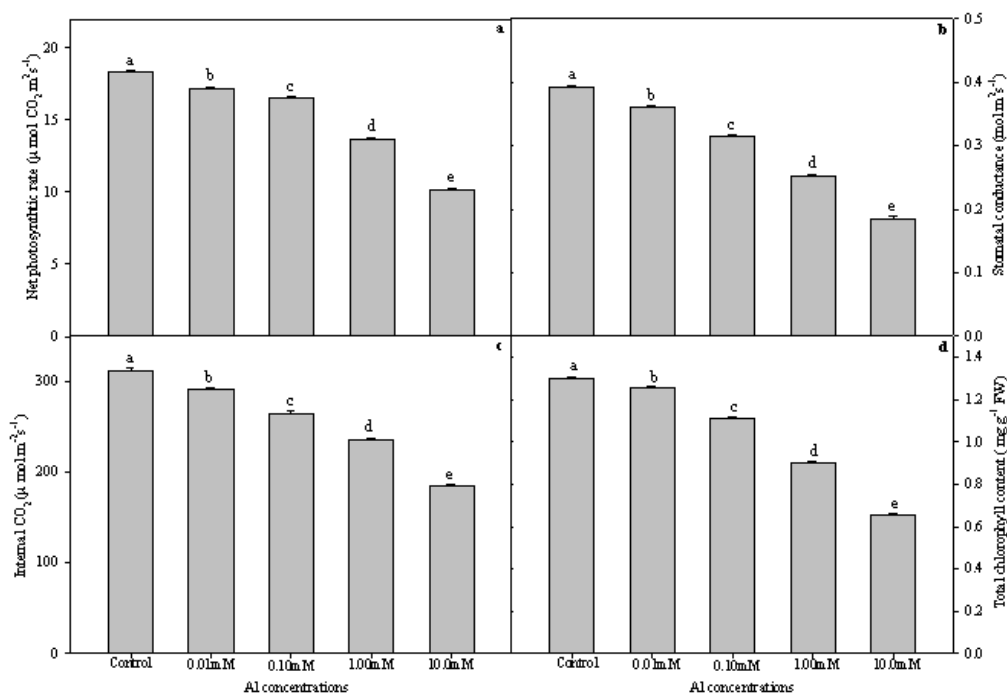
Fig 1. Effect of different concentrations of Al on net photosynthetic rate (a), stomatal conductance (b), internal \text{CO}_2 (c) and total chlorophyll content (d) of Artemisia annua L. Bars showing the same letter are not significantly different at p \leq 0.05 as determined by Duncan's multiple range test. Error bars ( \mp ) show SE
