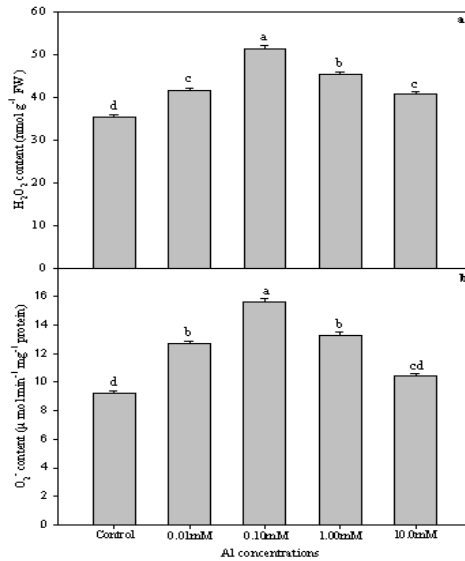
Fig. 4. Effect of different concentrations of Al on H 2 O 2 (a) and O 2 - (b) contents of Artemisia annua L. Bars showing the same letter are not significantly different at p \leq 0.05 as determined by Duncan's multiple range test. Error bars ( \uparrow ) show SE
