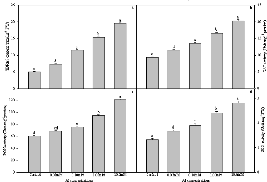
Fig. 3. Effect of different concentrations of Al on TBRAS content (a), CAT (b), POX (c) and SOD (d) activities in leaves of Artemisia annua L. Bars showing the same letter are not significantly different at p \leq 0.05 as determined by Duncan's multiple range test. Error bars ( \tau ) show SE
