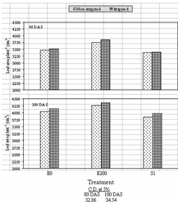
Fig. 1. Effect of ethrel (E: 0 or 200 µl/L) or silver thiosulphate (S: 1 mM) at 60 days after sowing (DAS; flowering stage) on leaf area plant -1 (cm 2 ) of mustard ( Brassica juncea L.) cultivar Alankar grown with basal 80 kg N ha -1 under irrigated and non-irrigated conditions at 80 and 100 DAS.
