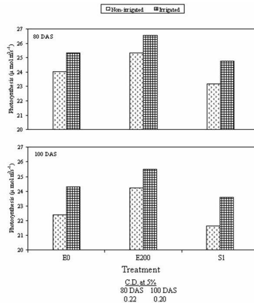
Fig. 2. Effect of ethrel (E: 0 or 200 µl/L) or silver thiosulphate (S: 1 mM) at 60 days after sowing (DAS ; flowering stage) on rate of photosynthesis (µ mol m -2 s -1 ) of mustard ( Brassica juncea L.) cultivar Alankar grown with basal 80 kg N ha -1 under irrigated and non-irrigated conditions at 80, and 100 DAS.
