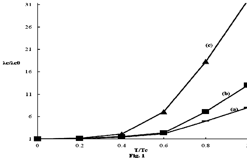
Fig1. The variation of \lambda_c/\lambda_{c0} vs T/T_c with (a) t_{11} = 200 meV (solid line), (b) t_{11} = 250 meV (solid square), (c) t_{11} = 300 meV (solid triangle). The other parameters are n_{ab} = 0.085 , t_{\perp} = 20 meV, \tilde{U} = -600 meV
