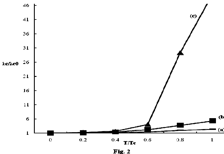
Fig 2. The variation of \lambda_c/\lambda_{c0} vs T/T_c with (a) t_{\perp} = 20 meV (solid line), (b) t_{\perp} = 40 meV (solid square), (c) t_{\perp} = 20 meV (solid triangle). The other parameters are n_{ab} = 0.085 , t_{11} = 200 meV, keeping U+W = -600 meV.
