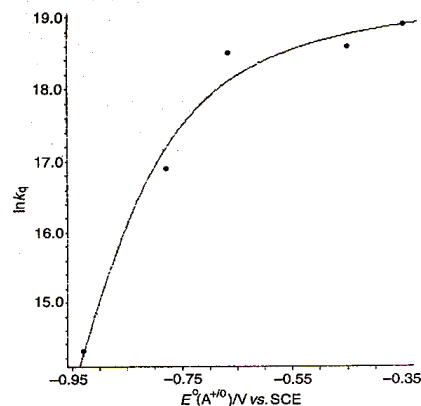
Fig 6. Plot of k_q vs. E^{\circ}(A^{+/0}) for the oxidative quenching of complex 2 by pyridinium acceptors in degassed acetonitrile: (•) experimental data; (-) fitted curve.
