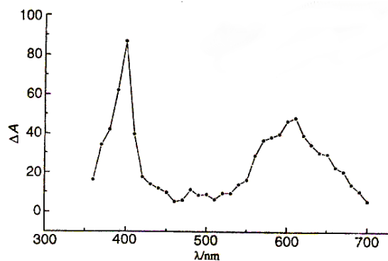
Fig 9. Transient difference absorption spectrum recorded 20 \mu\text{s} after 355 nm excitation of a degassed acetonitrile solution of complex 2 ( 10^4 mol \text{dm}^{-3} ) and N,N'-dimethyl-4,4'-bipyridinium hexafluorophosphate ( 10^{-3} mol \text{dm}^{-3} ) at room temperature.
