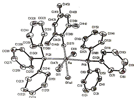
Fig 2. A perspective view of [Re(CC 6 H 2 Me 3 -2,4,6)(PPh 3 ) 2 (CO)-(H 2 O)Cl] + .
