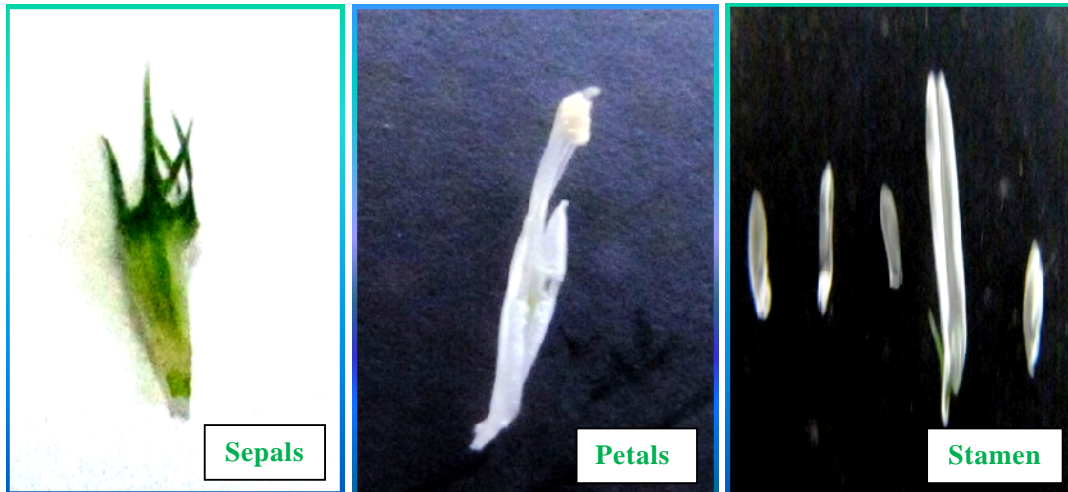
Figure 2: Sepals, petals and stamen of T. alexandrinum flower
