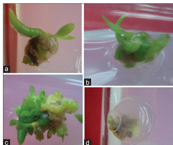
Figure 1: Morphogenetic response of encapsulated protocorm-like bodies (PLBs) of Rhynchosstylis retusa under the effect of ascorbic acid (5, 10, 15, and 20 mM): (a) Lush-green leaves with high chlorophyll content (5 mM); (b) PLBs conversion (10 mM); (c) excessive somatic embryogenesis and low chlorophyll content (15 mM); (d) growth inhibition (20 mM)
