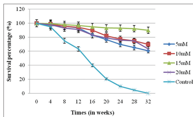
Graph 1: Survival percentage of encapsulated protocorm-like bodies in Rhynchosstylis retusa under the effect of ascorbic acid (5, 10, 15, and 20 mM) up to 32 weeks
